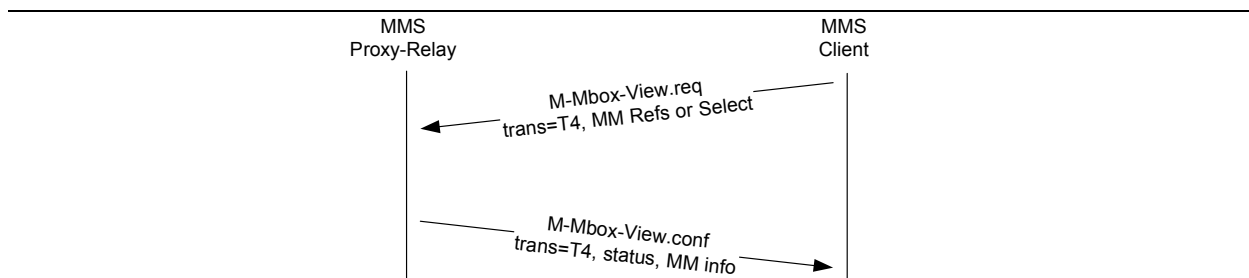
Figure 18. Example MMS Mbox-View Transaction
