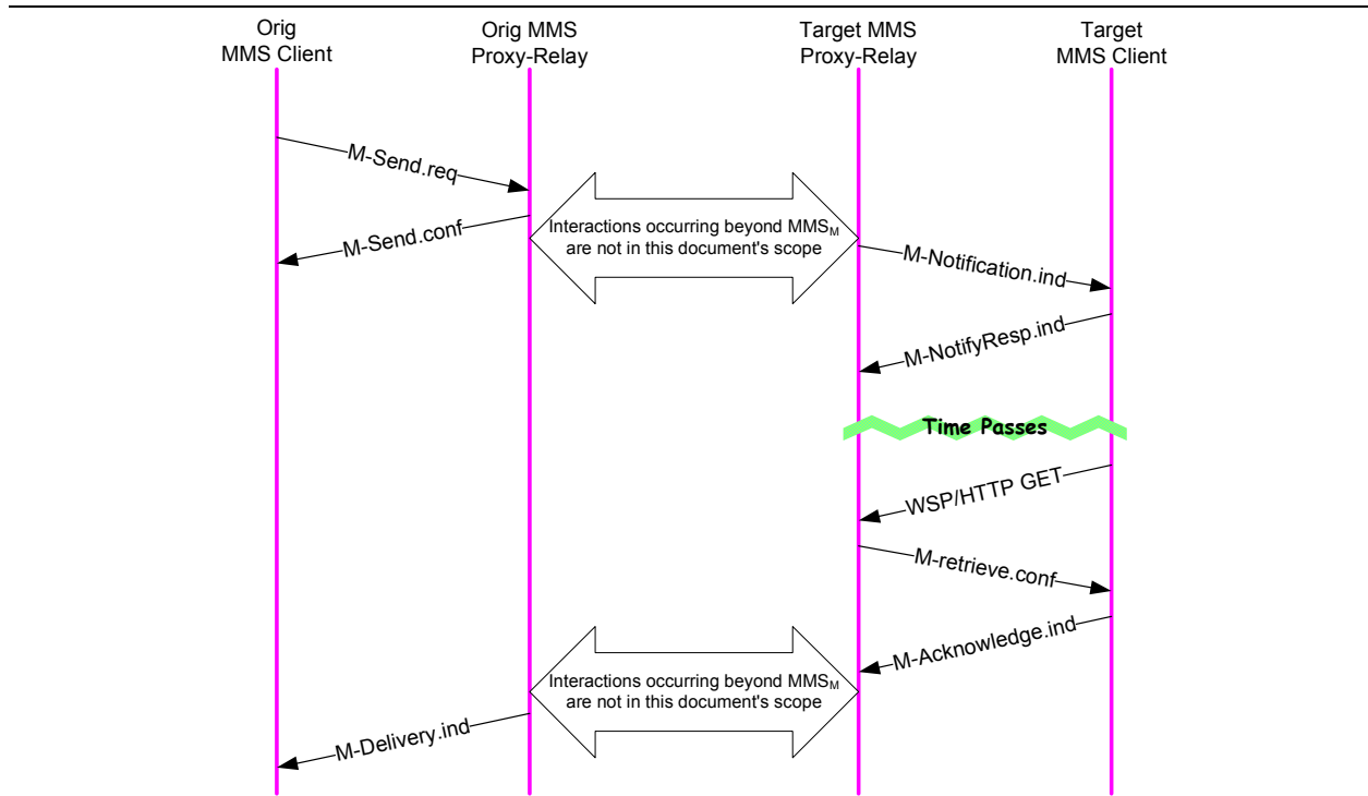
Figure 7: Example MMS Transaction Flow – Deferred Retrieval
