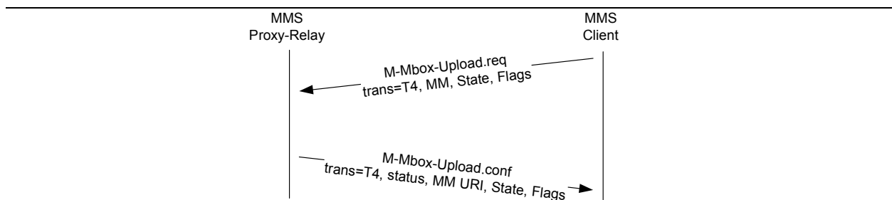
Figure 23: Example MMS Upload to MMBox Transaction
