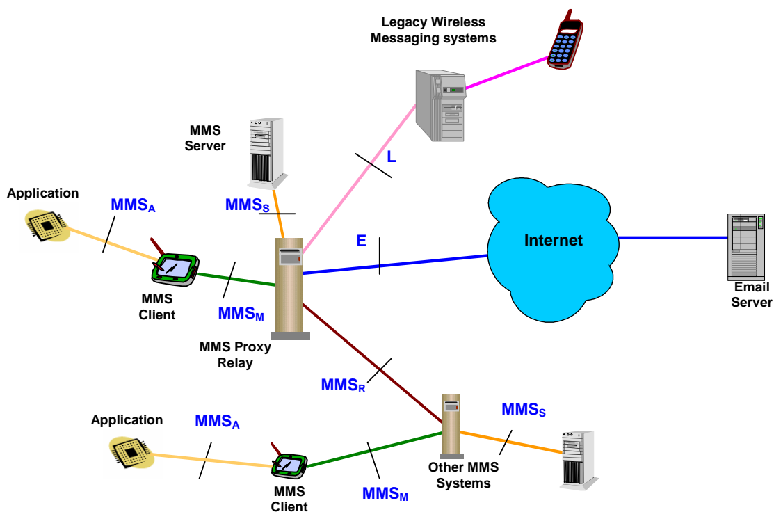
Figure 2: MMS Network Representation
