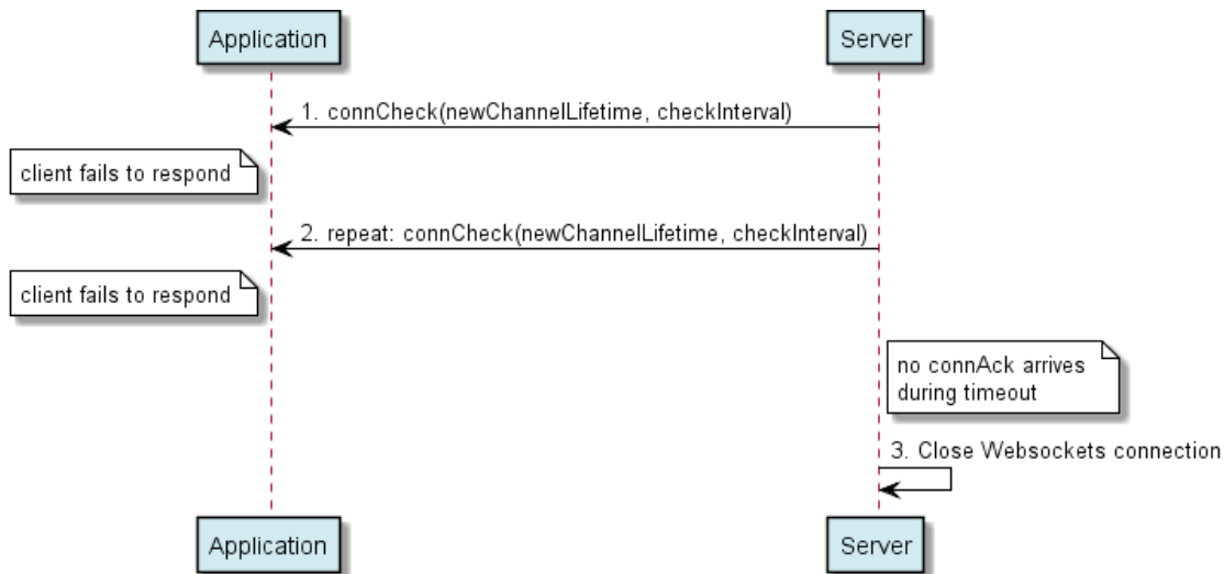
Figure 17 Unsuccessful server-initiated ConnCheck/ConnAck for session keep-alive
