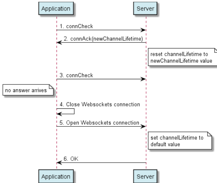
Figure 15 Client-initiated ConnCheck/ConnAck for session keep-alive
