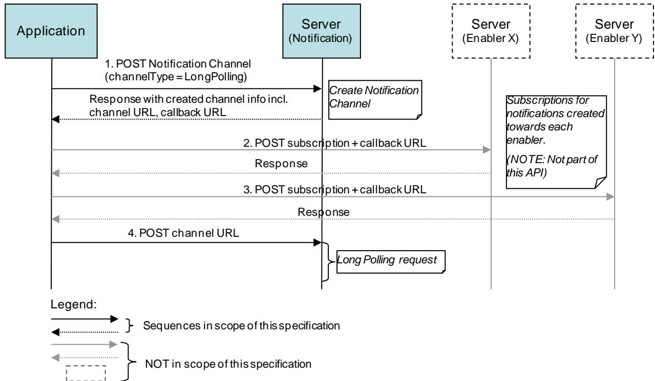
Figure 2 Create Notification Channel
