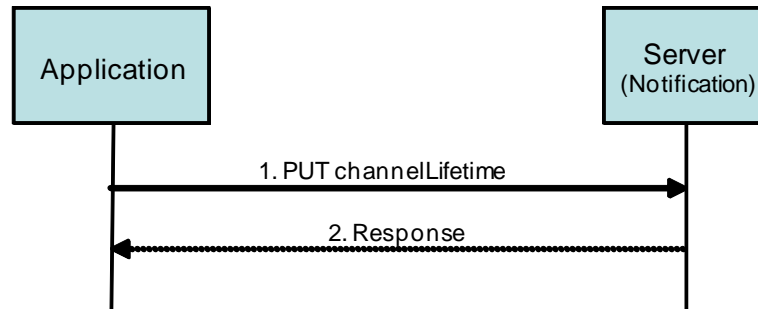
Figure 14 Notification Channel refresh
