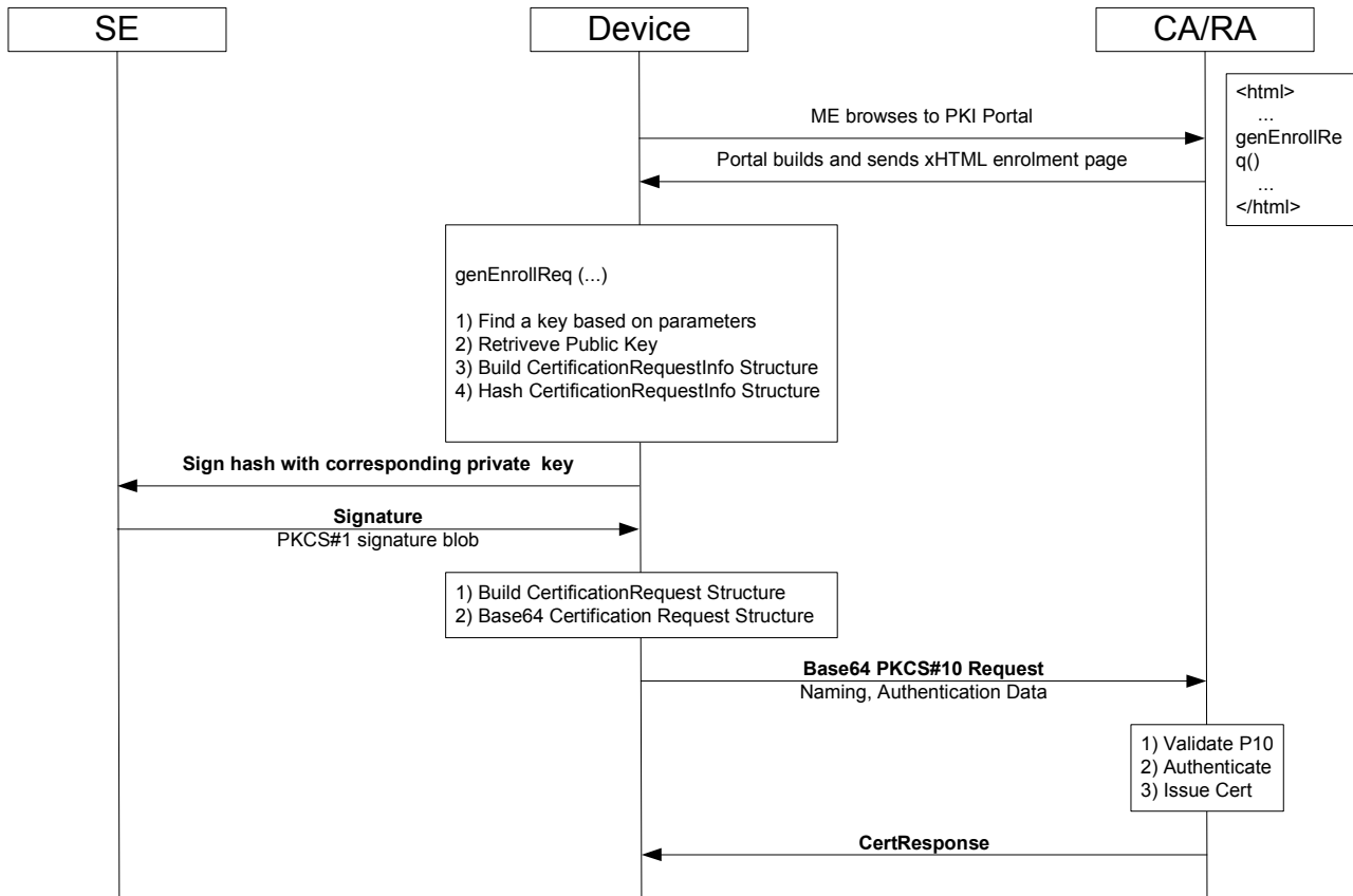
Figure 6 - genEnrollReq dataflow
