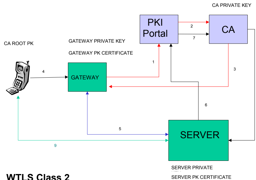
Figure 1 - WTLS Class 2 WPKI
