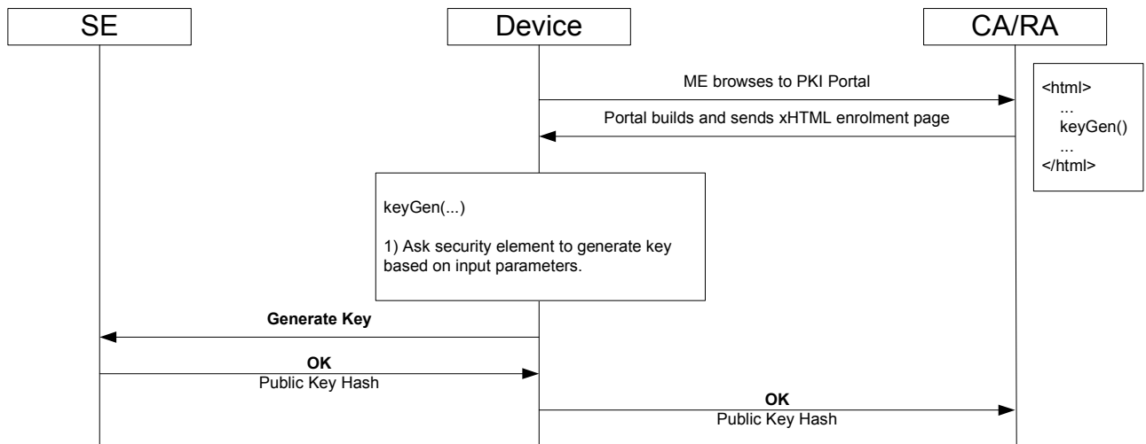
Figure 5 - keyGen Dataflow
