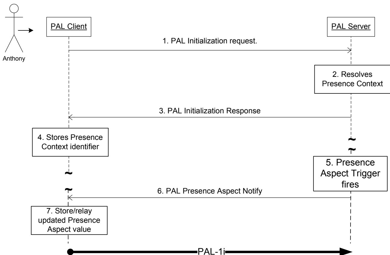
Figure 5: Receiving a Predefined Action corresponding with a Presence Trigger
