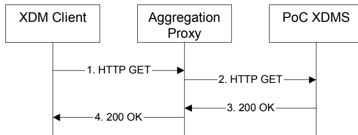
Figure B.1- XDM Client obtains a particular PoC Group document
