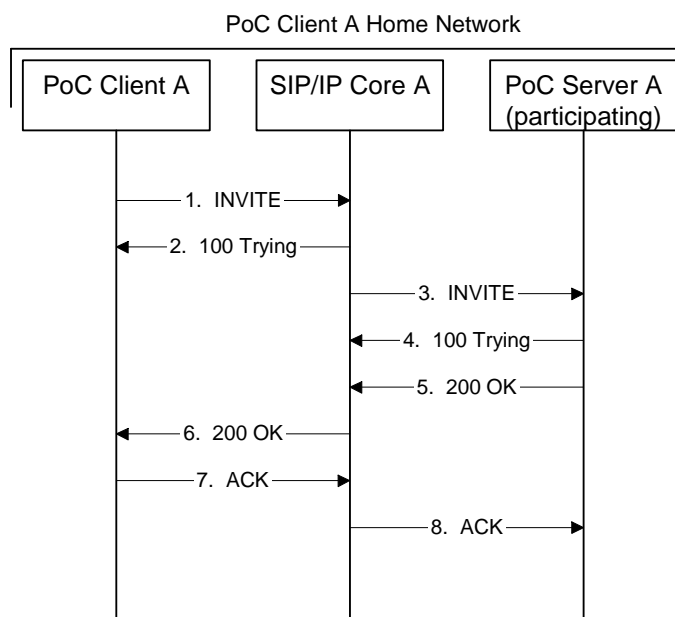
Figure 4: PoC Client A initiates a Pre-established Session
