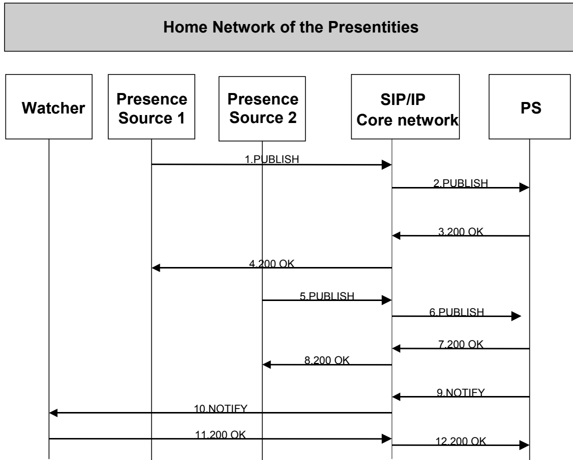
Figure 11- Aggregating published presence information from multiple sources
