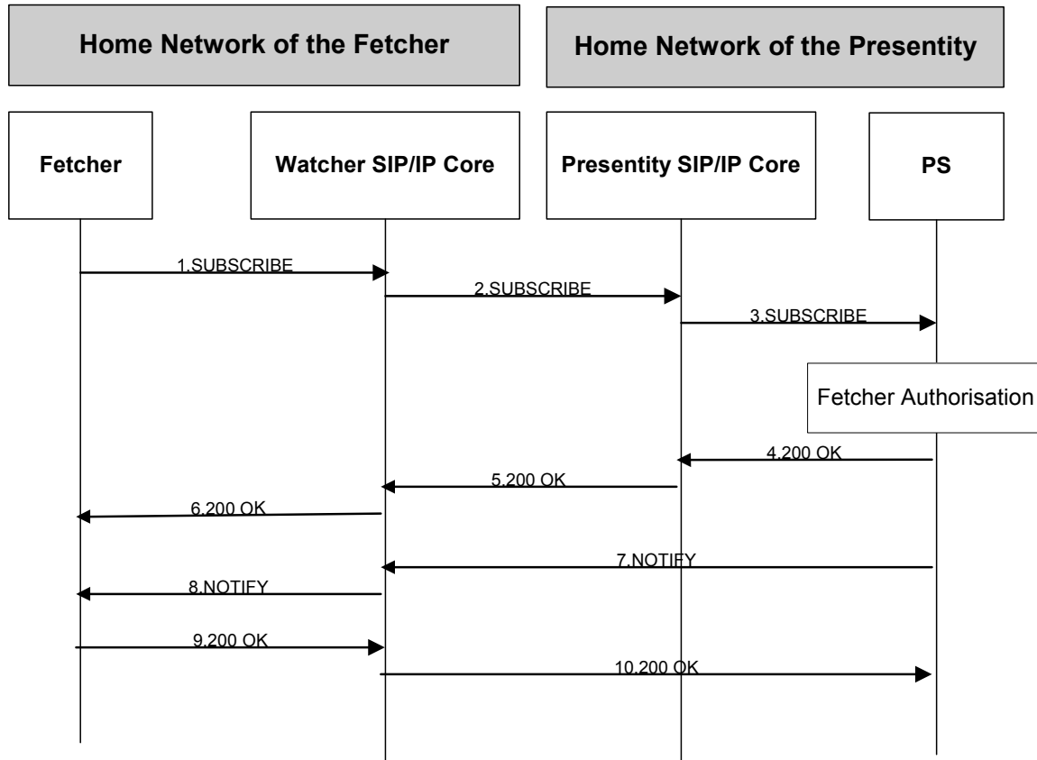
Figure 13 - Fetching presence information state (fetcher and presentity are in different networks)
