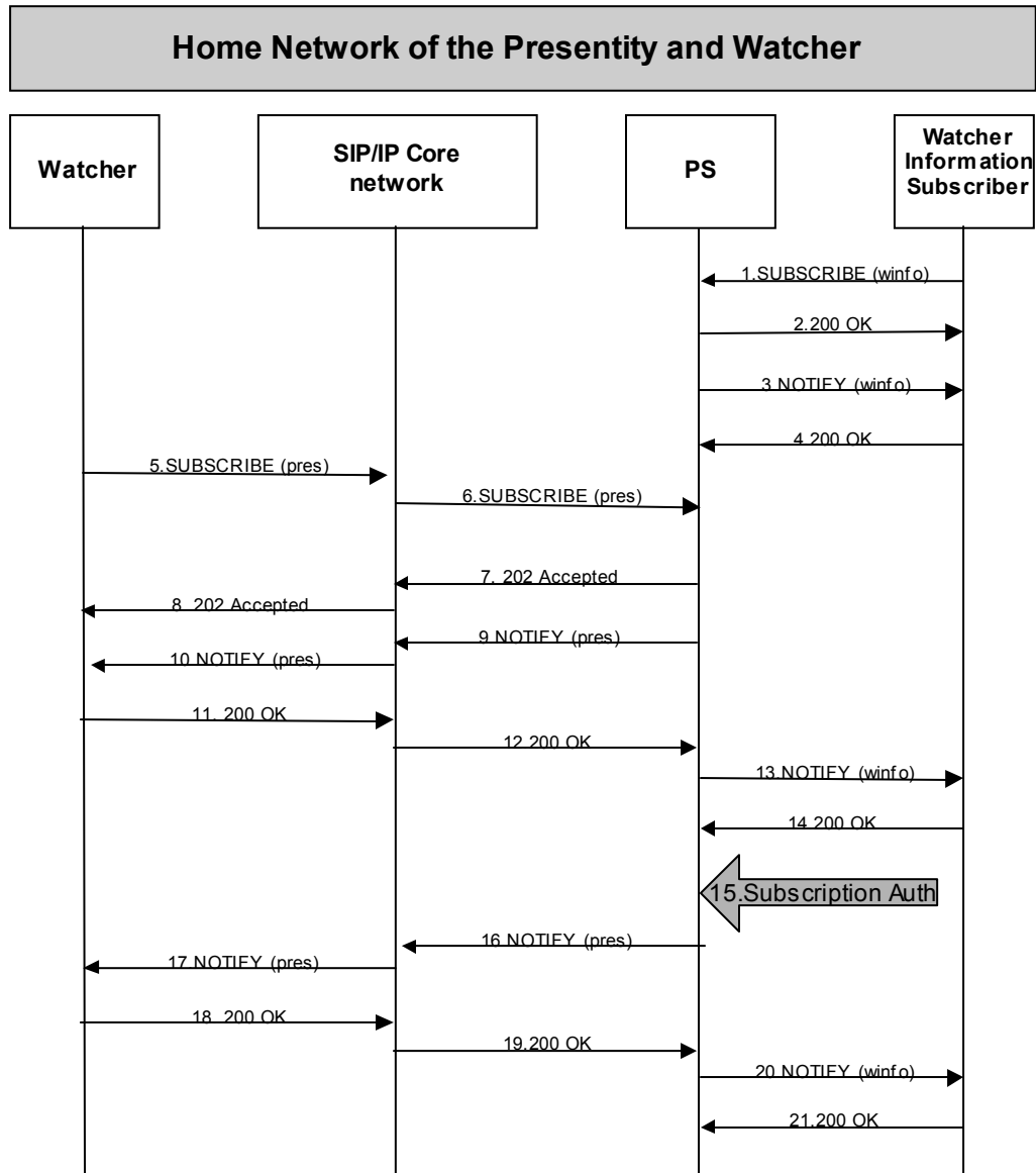
Figure 23- Watcher Information (Subscriptions/Notifications)
