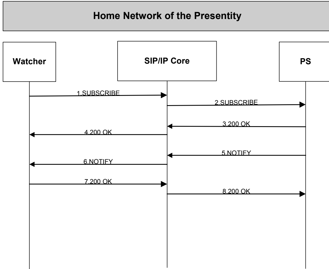
Figure 20 - Subscription Filters
