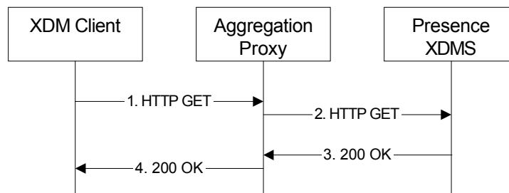
Figure B.1- XDM Client obtains Presence Authorisation Rules
