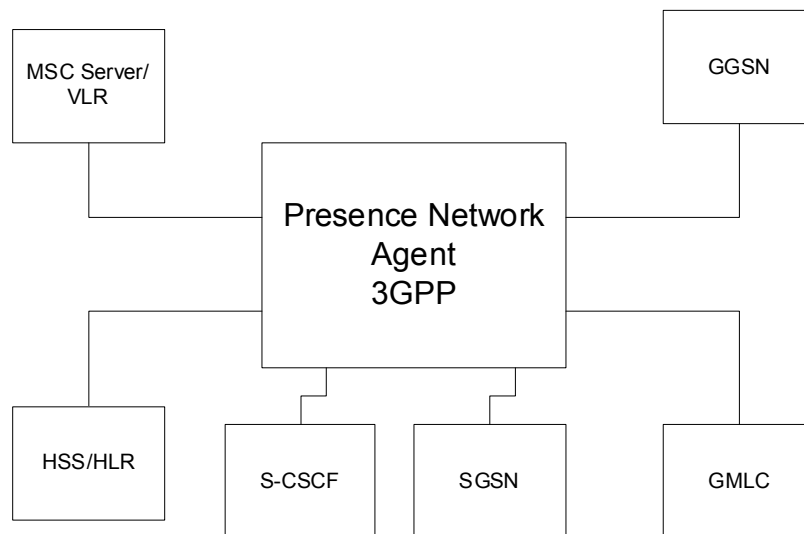
Figure 1-PNA in 3GPP
