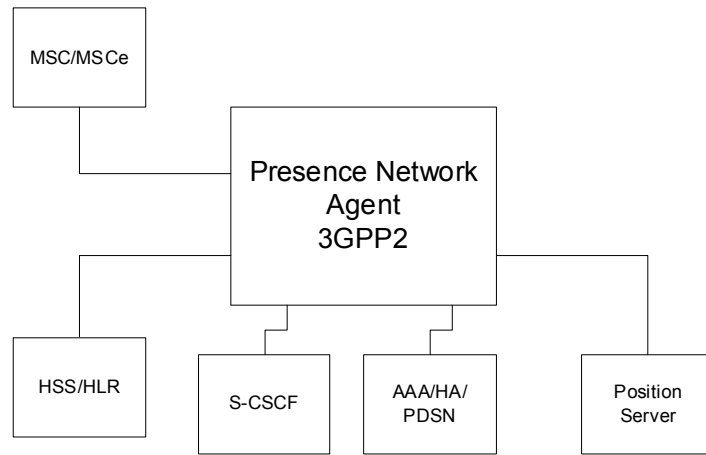
Figure 2-PNA in 3GPP2
