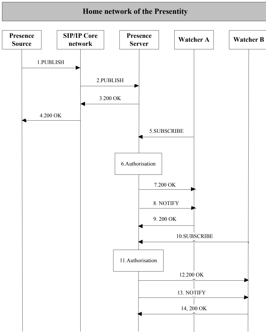
Figure 22 - Sending different Presence Information to different Watchers
