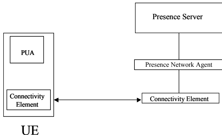
Figure 3-PNA in a non-3GPP/3GPP2 architecture.
