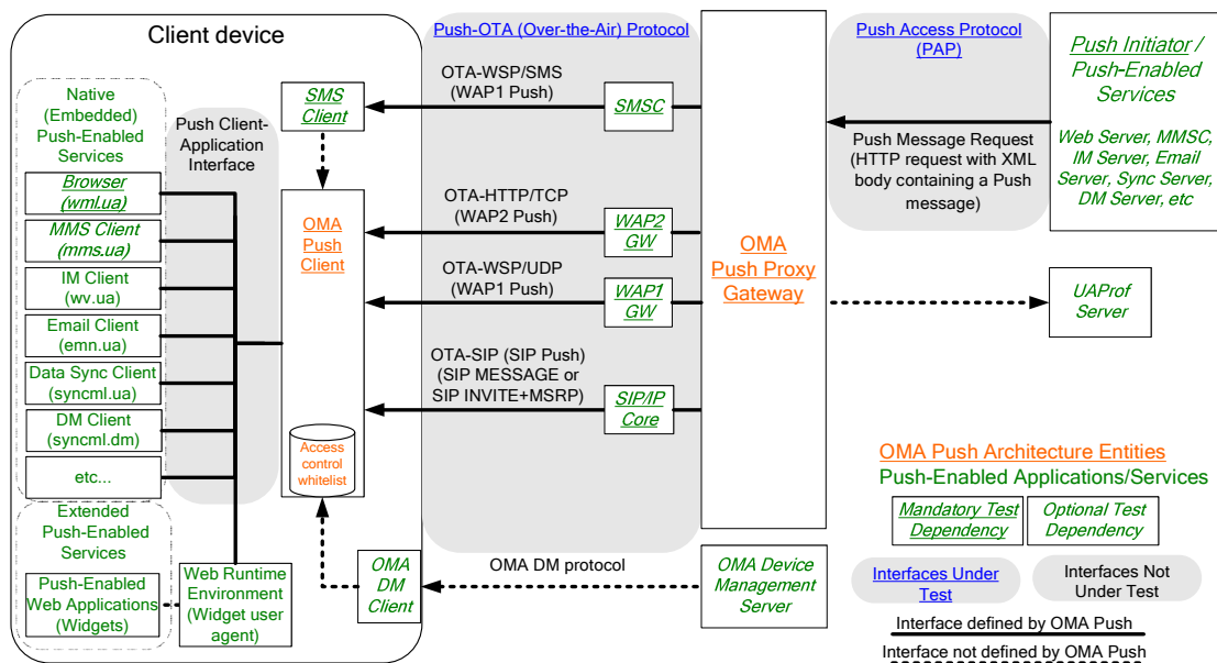
Figure 1 OMA Push Test Configuration
