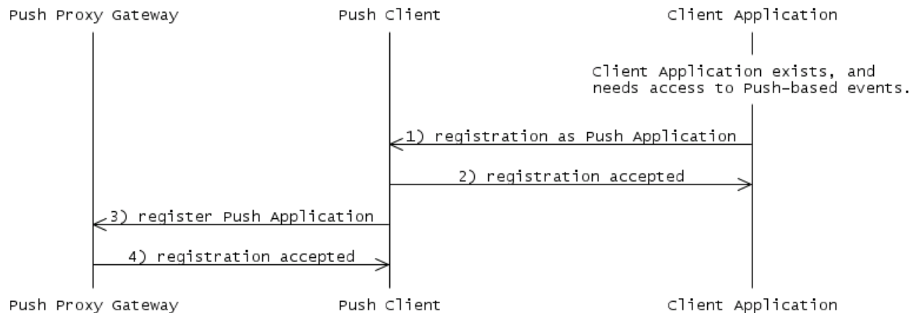
Figure 9 Push Client Registration
