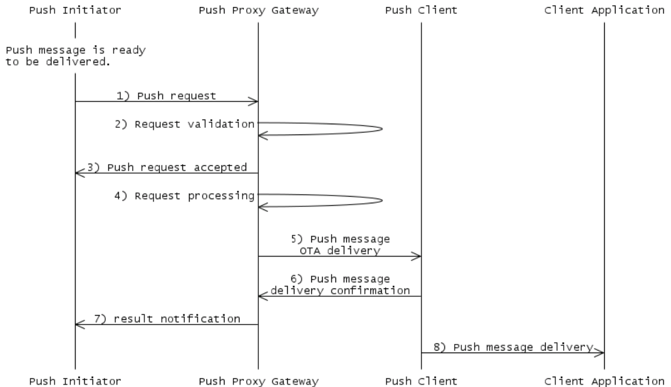
Figure 11 Push Message Delivery
