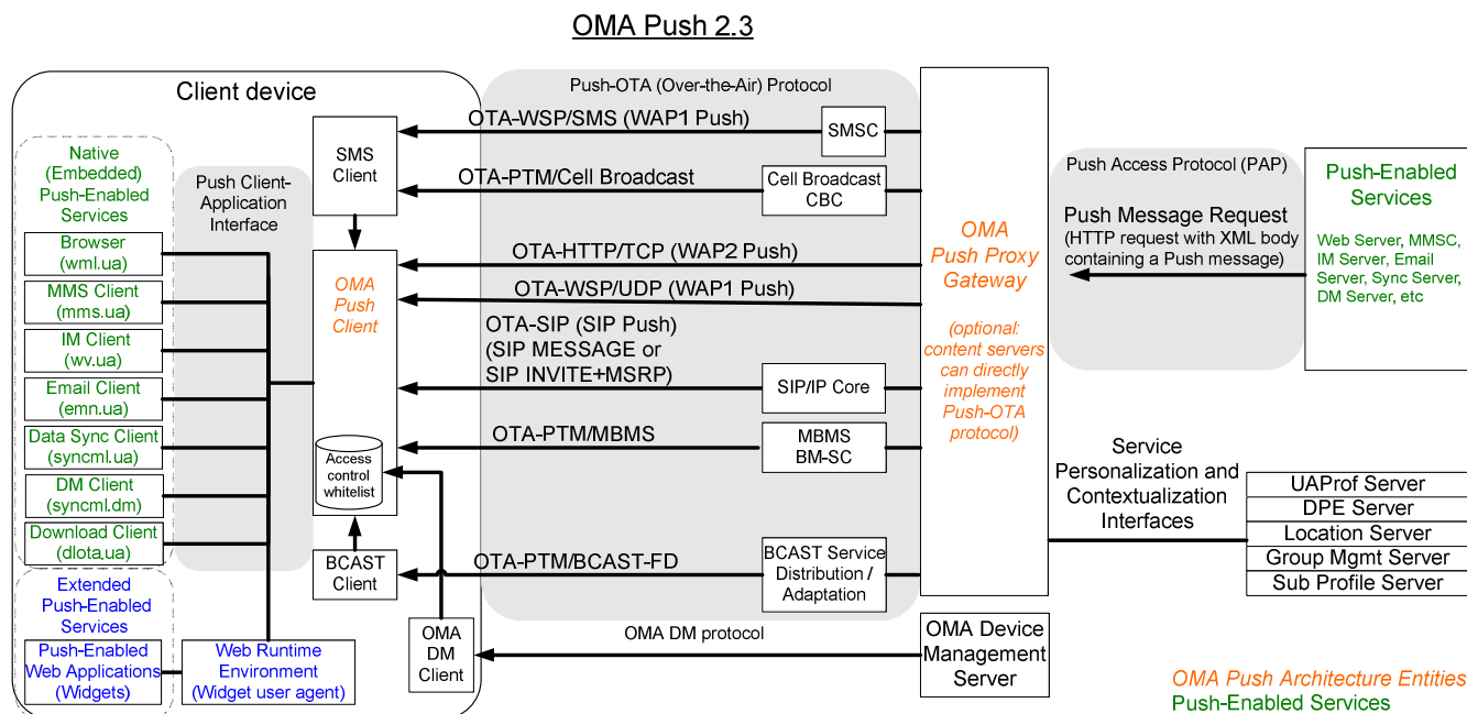
Figure 3 End-to-End Push Framework
