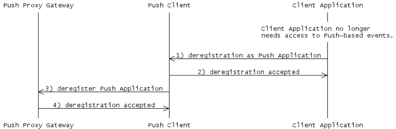
Figure 10 Push Client Deregistration
