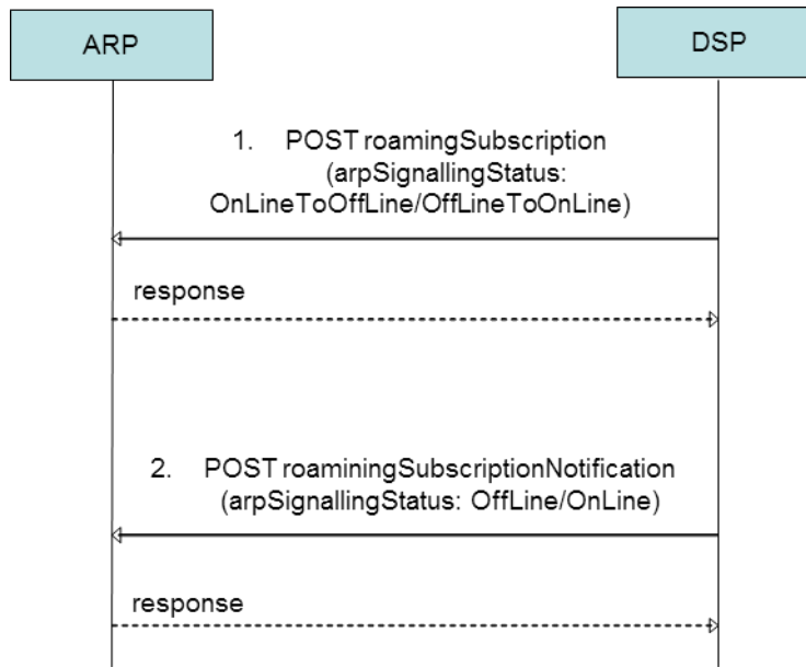
Figure 5 Signalling status change – DSP initiated
