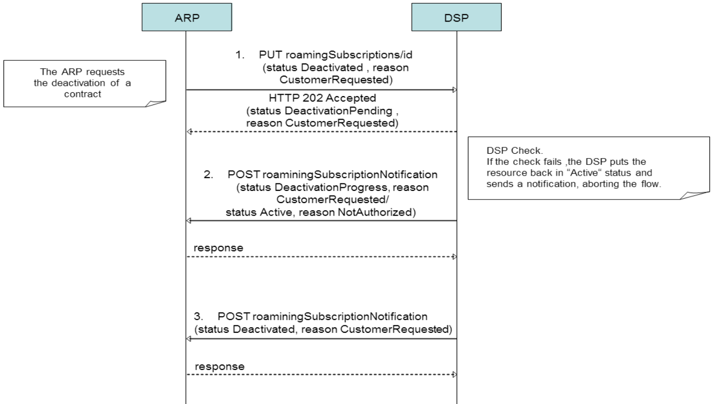
Figure 9 Deactivation of roaming subscription
