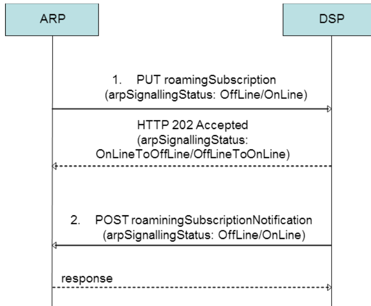
Figure 4 Signalling status change – ARP initiated
