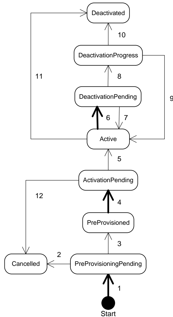
Figure 10 Roaming subscription state machine
