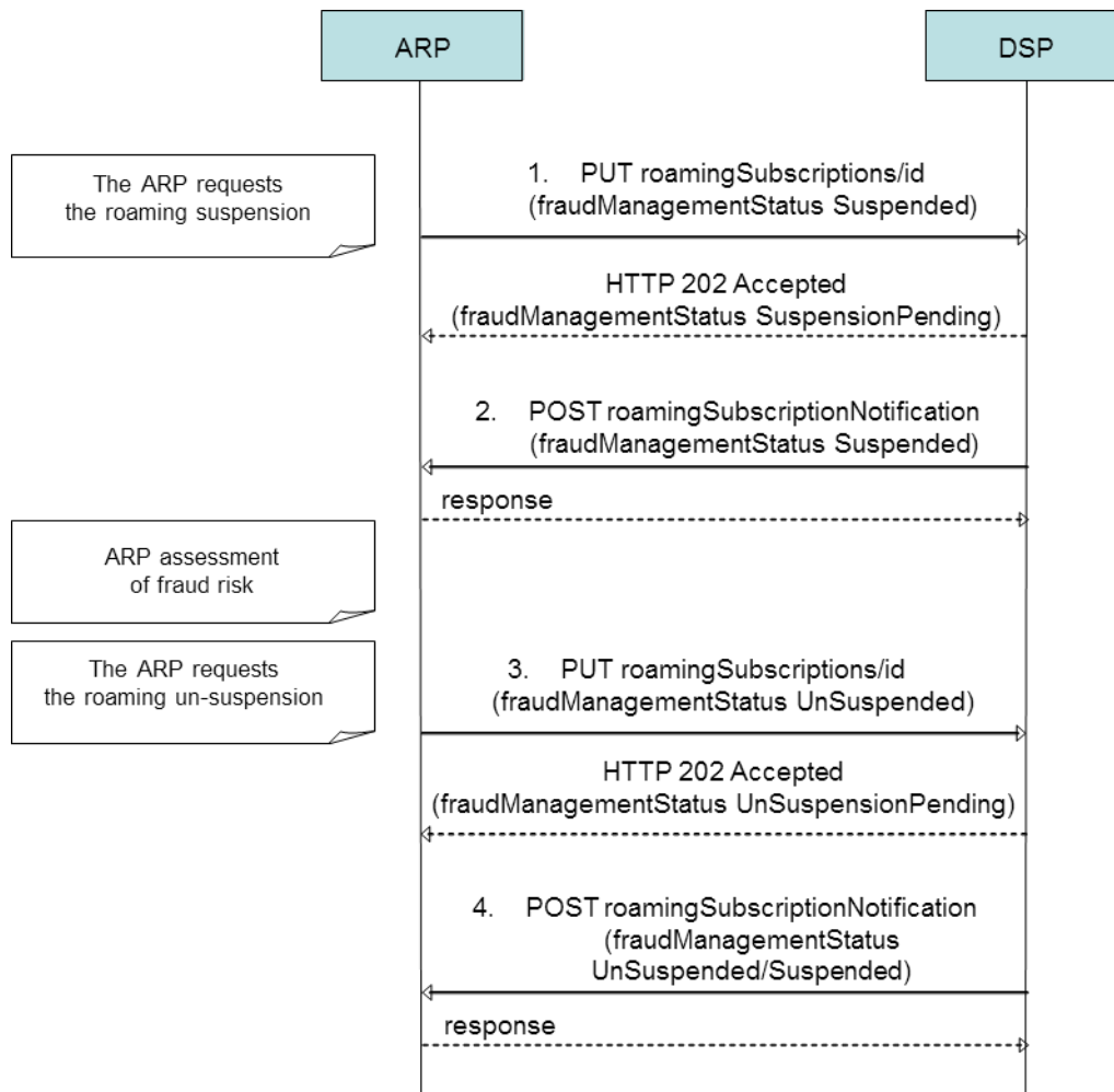
Figure 7 Roaming subscription suspension and un-suspension
