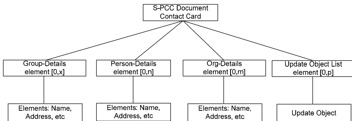
Figure 2 High Level S-PCC Document Structure
