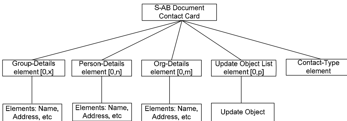
Figure 1 High Level S-AB Document Structure
