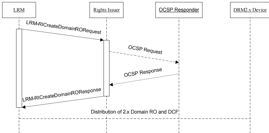
Figure 4 – The 2-pass LRM-RI Create Domain RO Protocol
