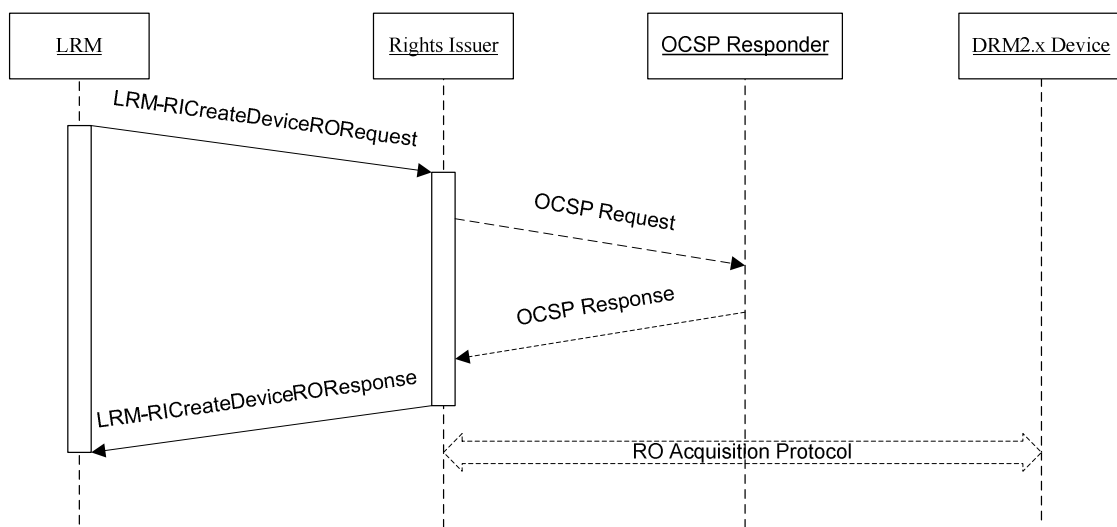
Figure 3 – The 2-pass LRM-RI Create Device RO Protocol
