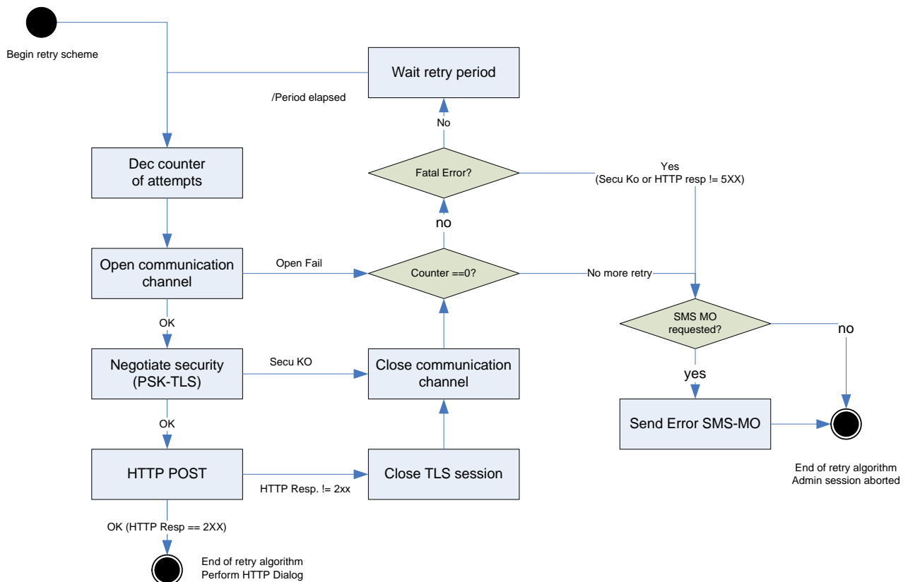
Figure 4: Retry algorithm
