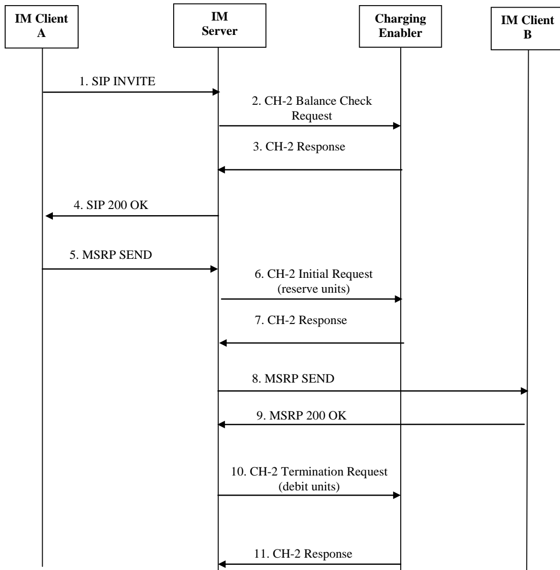
Figure 18: Online Charging for Large message
