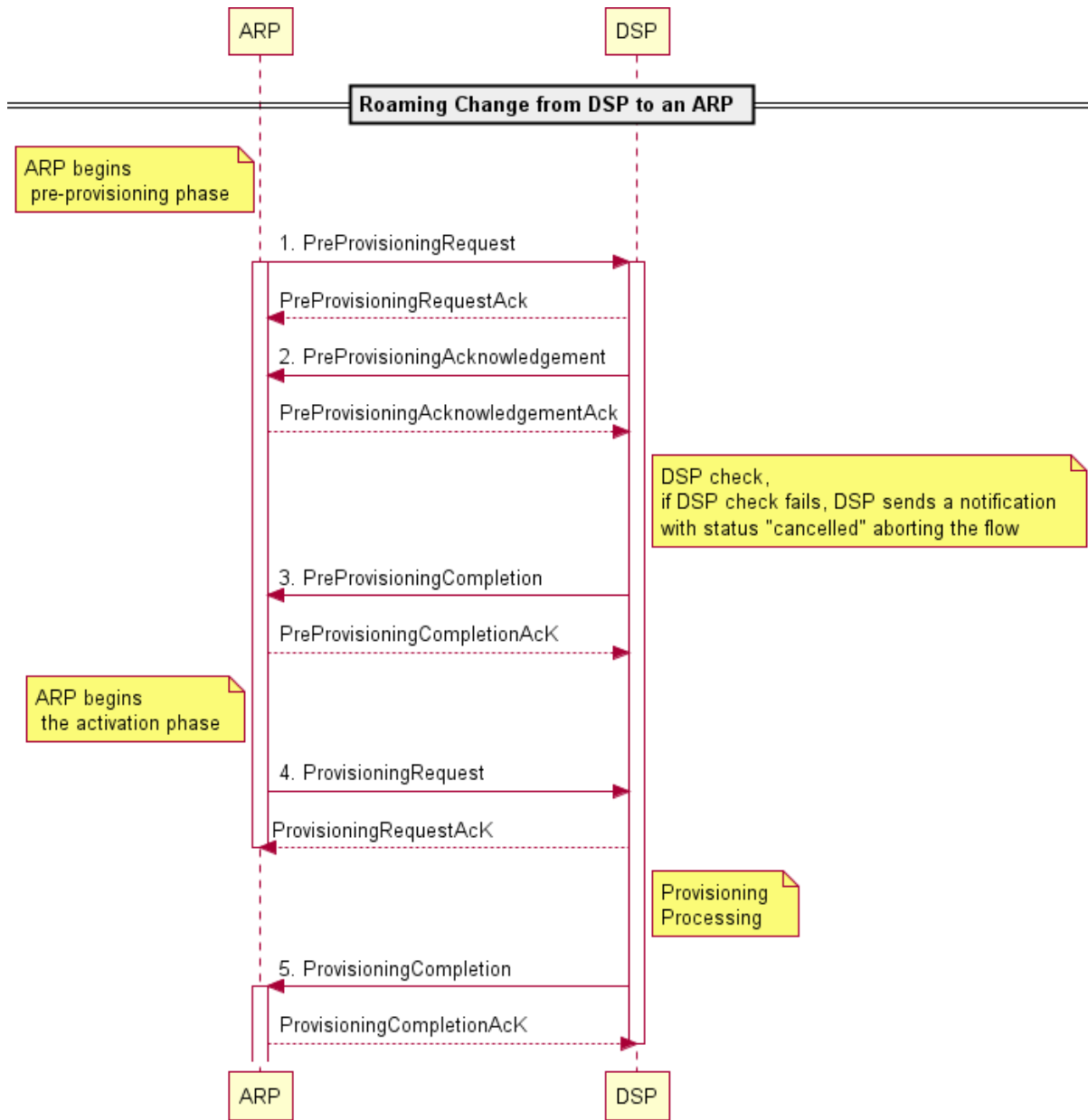
Figure 1: Roaming subscription activation
