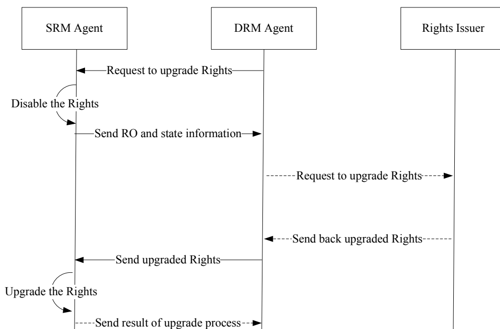
Figure 9: Sequence Diagram – SRM Rights upgrade
