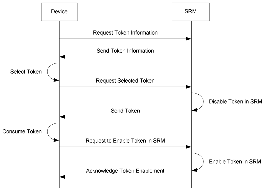
Figure 15: Sequence Diagram – Local Token Consumption
