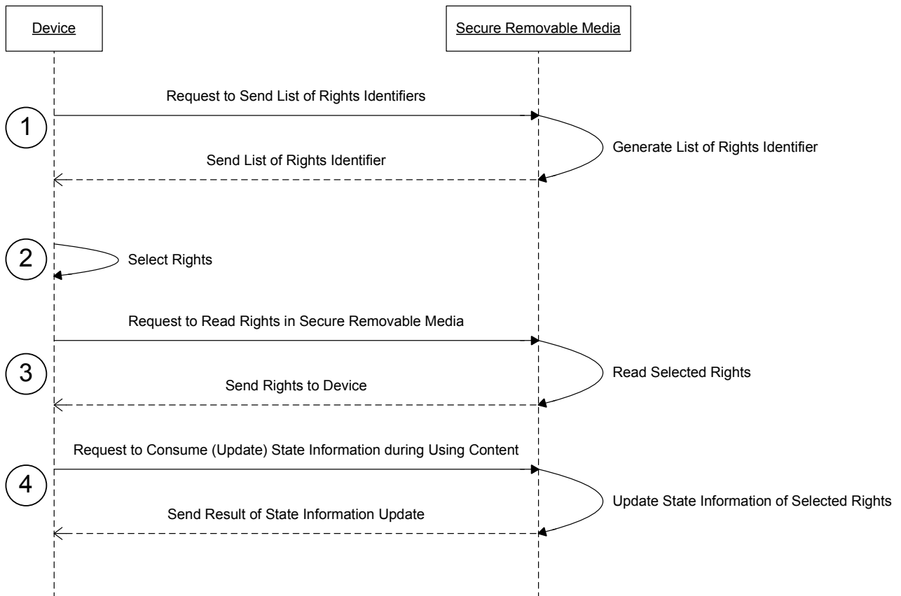
Figure 5: Sequence Diagram – Rights Consumption in SRM
