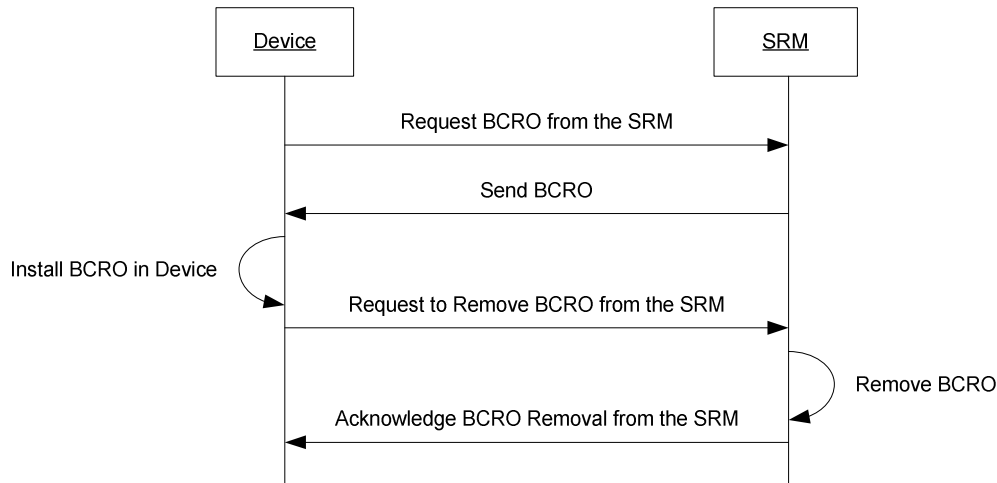
Figure 12: Sequence Diagram – BCRO Move from SRM to Device
