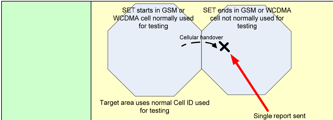
Figure 4: Case 4: SET leaves area
