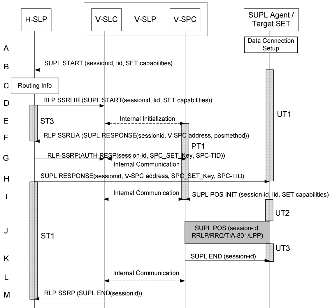
Figure 55: SET-Initiated Roaming with V-SPC Positioning Successful Case – Non-Proxy mode
