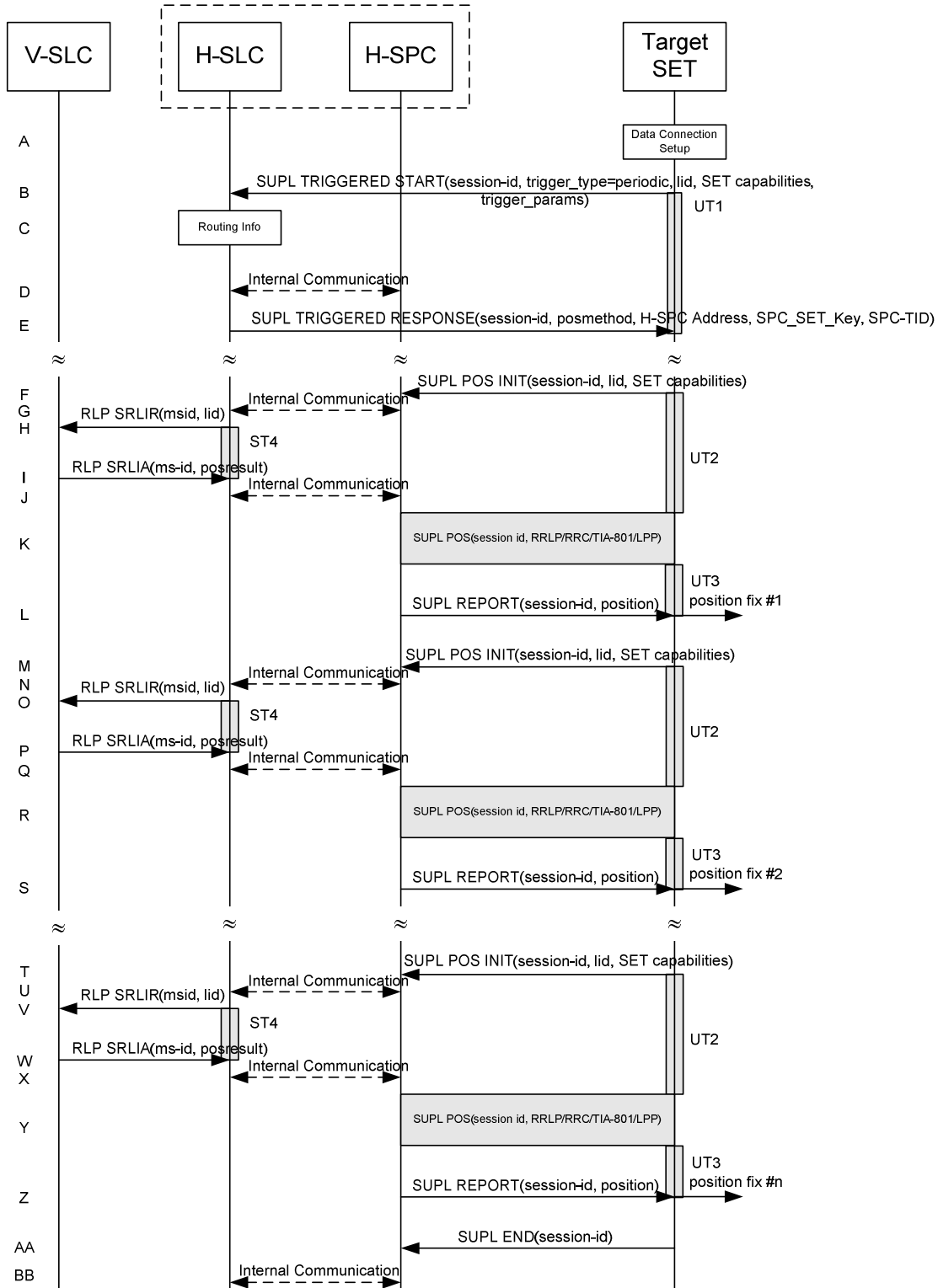
Figure 71: SET Initiated Periodic Trigger Service Roaming with H-SLP Positioning Successful Case – Non-Proxy Mode
