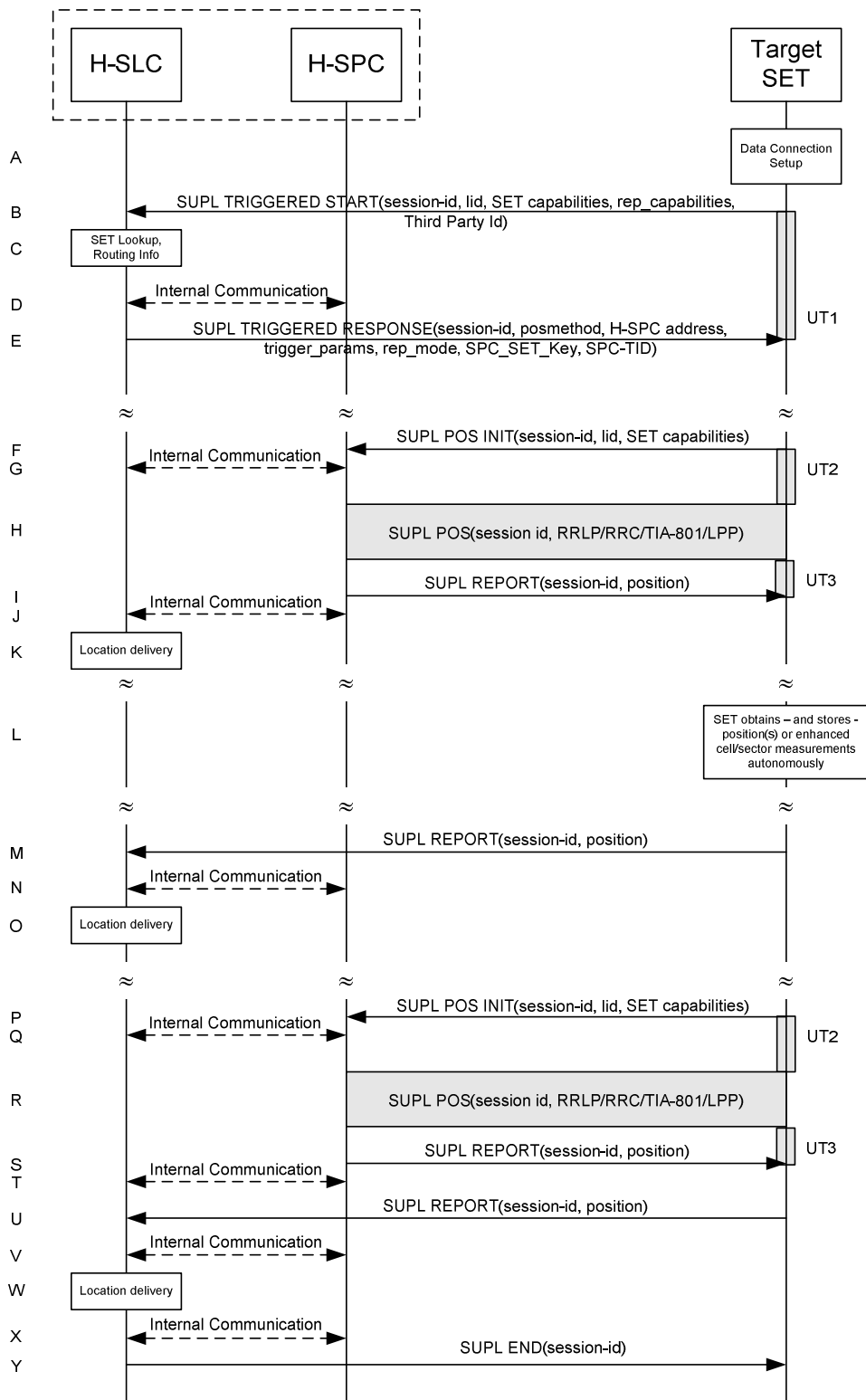
Figure 81: SET Initiated Periodic Location Request with transfer of the position result to 3rd party – non-roaming – non-proxy mode
