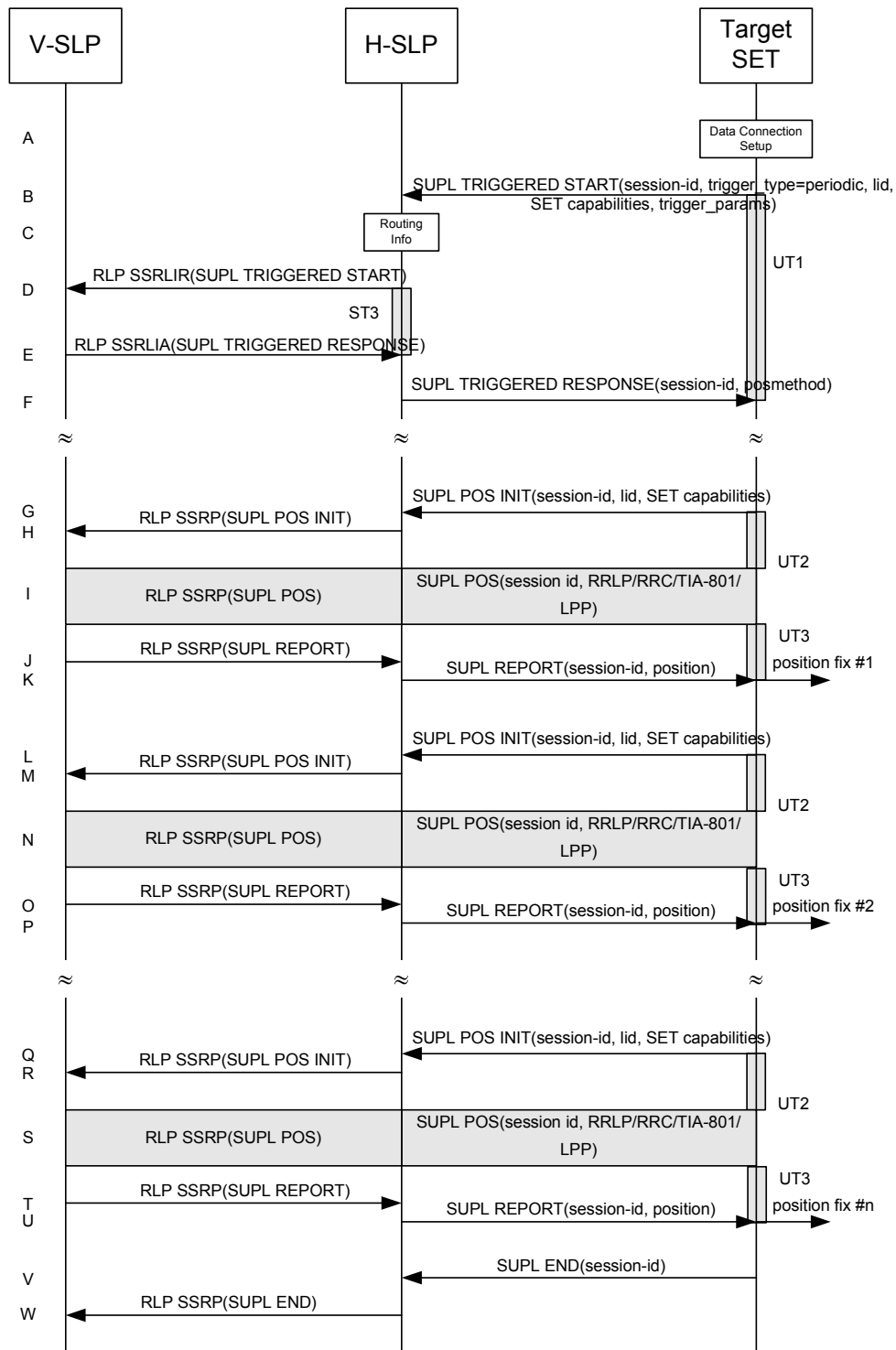
Figure 61: SET Initiated Periodic Trigger Service Roaming with V-SLP Positioning Successful Case – Proxy Mode
