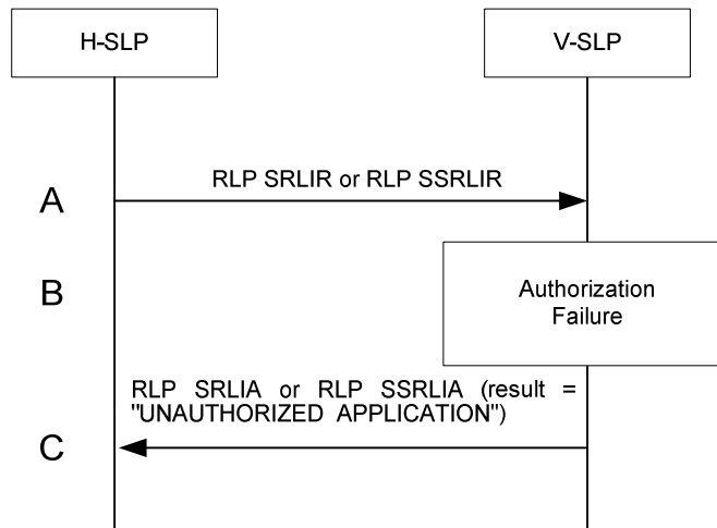
Figure 46: Network Initiated Authorization Failure V-SLP
