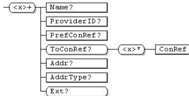
Figure 1: The OMA SUPL Management Object tree
