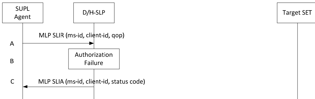
Figure 38: Network Initiated Authorization Failure D/H-SLP
