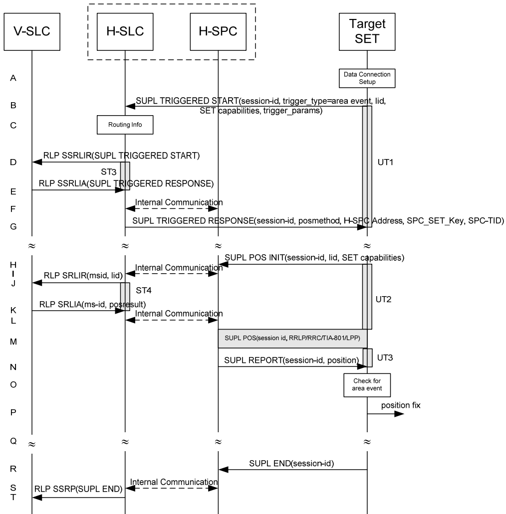
Figure 67: SET Initiated Area Event Trigger Service Roaming with H-SLP Positioning Successful Case – Non-Proxy Mode
