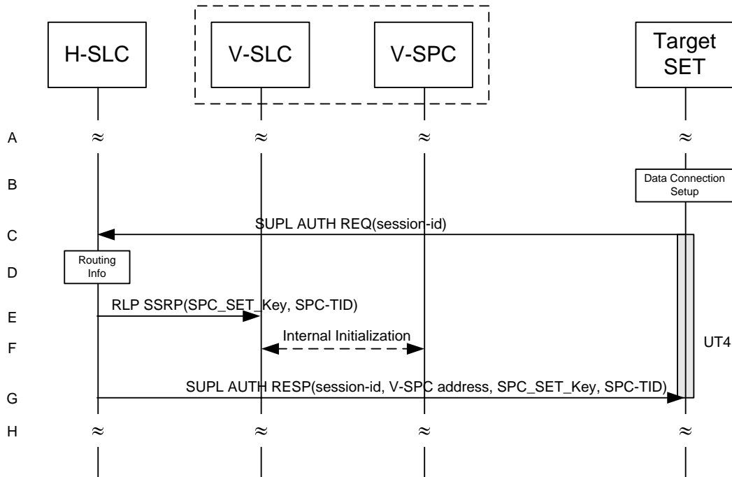
Figure 82: Key Refresh for Triggered Scenarios – roaming with V-SLP Positioning
