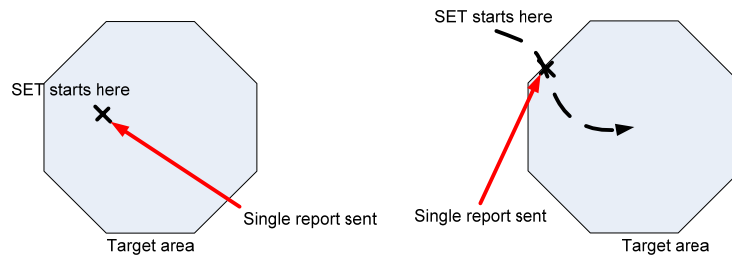
Figure 93: Single report when SET is inside area
