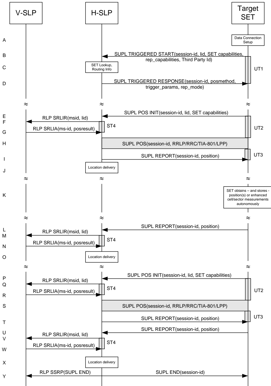
Figure 70: SET Initiated Periodic Location Request with transfer of the position result to 3rd party – roaming with H-SLP Positioning – proxy mode
