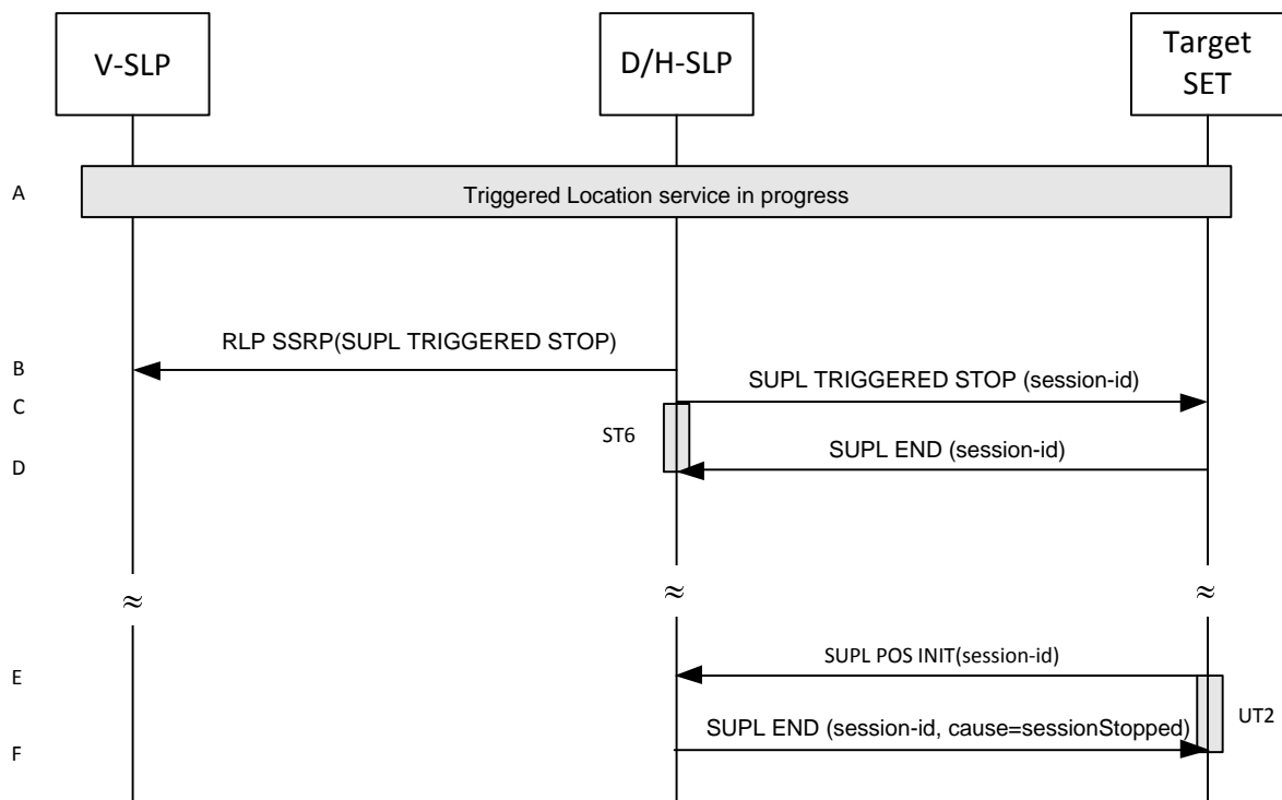
Figure 78: SET Initiated Triggered location, Network cancels the triggered location request
