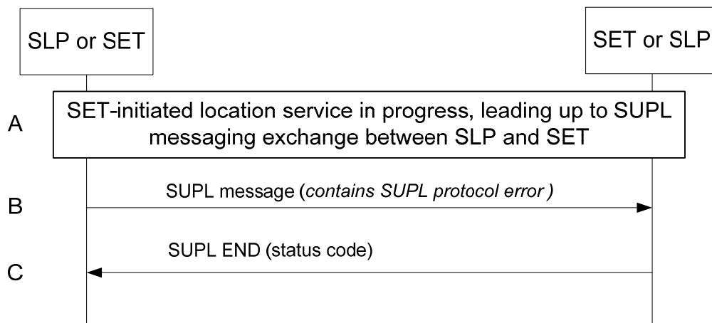
Figure 76: SET-Initiated Error SUPL Protocol Error
