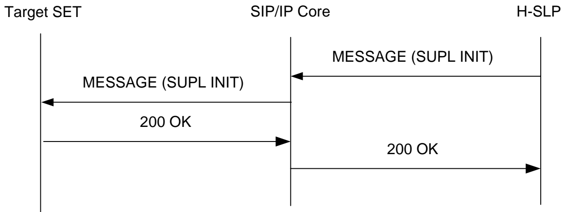
Figure 91: SIP Push Message flow
