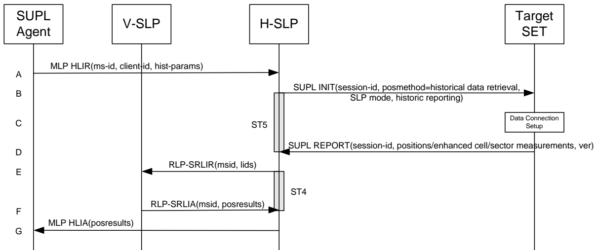
Figure 29: Retrieval of historical positions and/or enhanced cell/sector measurements – roaming
