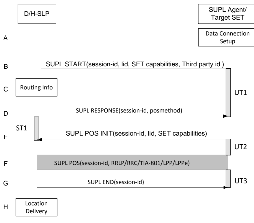
Figure 74: SET Initiated Location Request of Transfer Location to Third party
