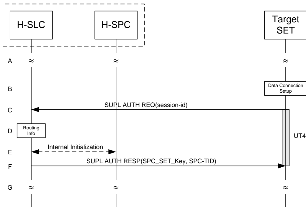
Figure 81: Example Figure Key Refresh for Triggered Scenarios – non-roaming
