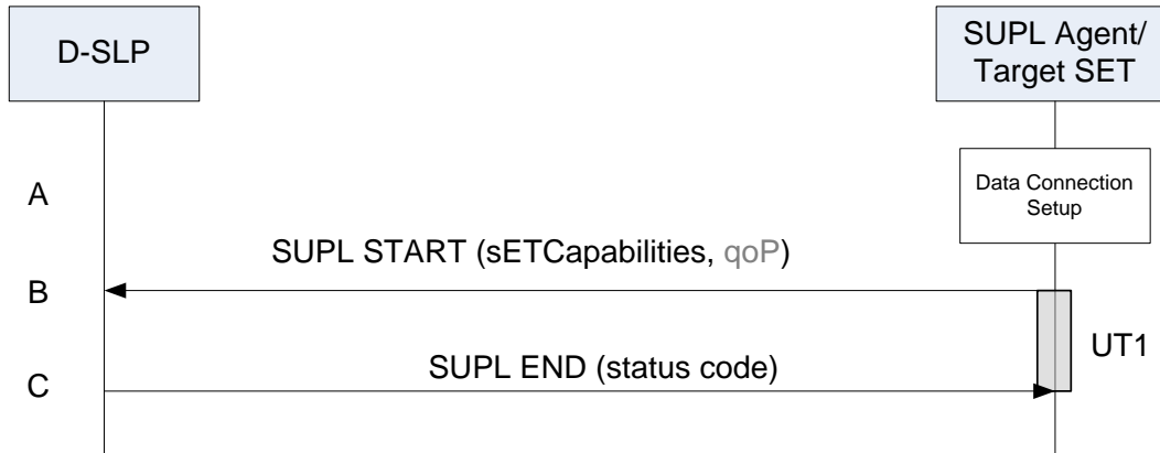
Figure 80: Invalid SET Access to a D/SLP
