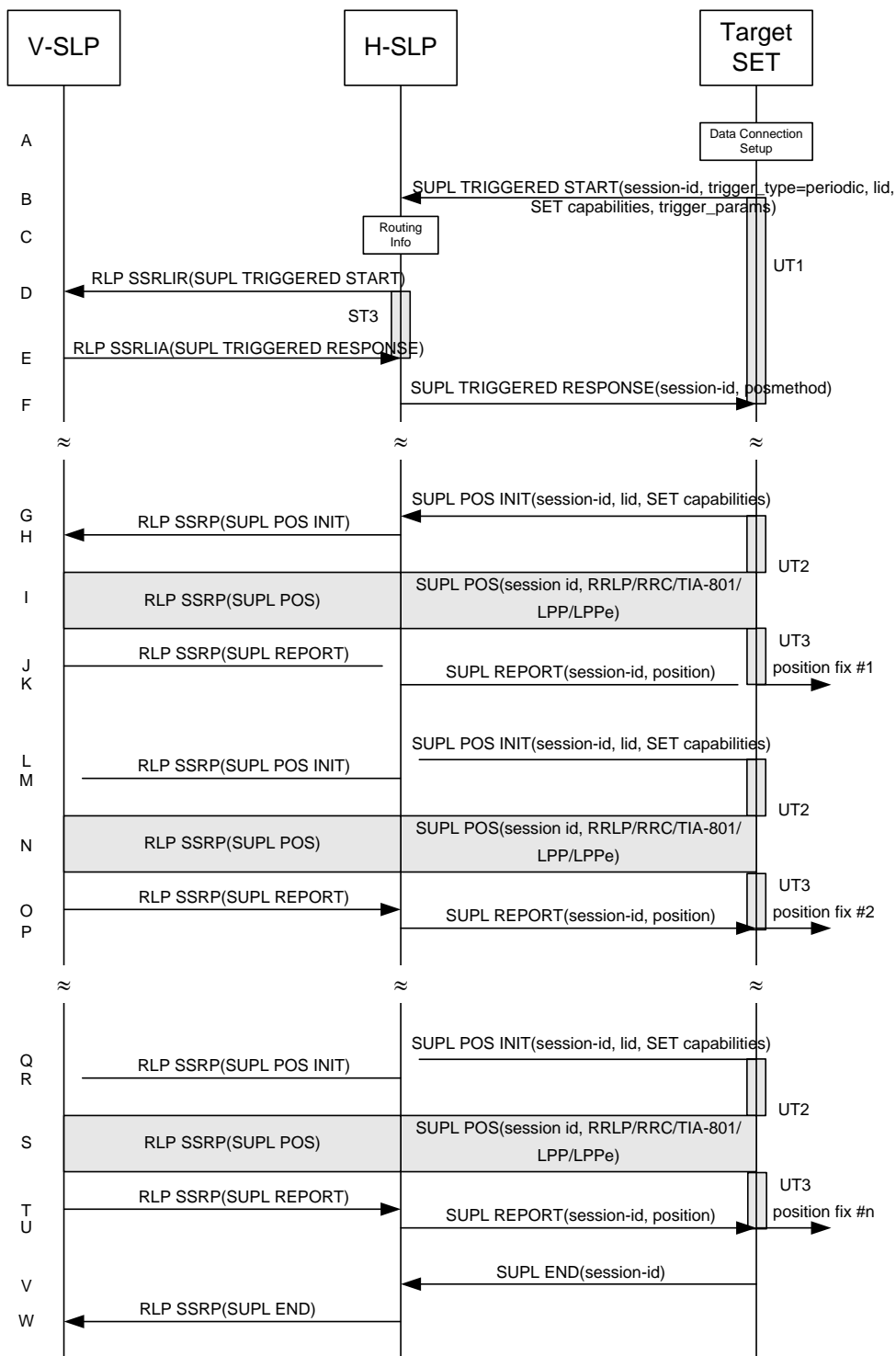
Figure 57: SET Initiated Periodic Trigger Service Roaming with V-SLP Positioning Successful Case – Proxy Mode
