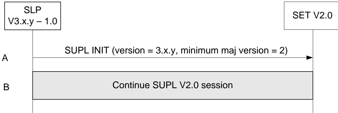
Figure 84: Network Initiated – SLP supports SUPL versions between 1.0 and 3.x.y and the requested service is V2.0 compatible.
