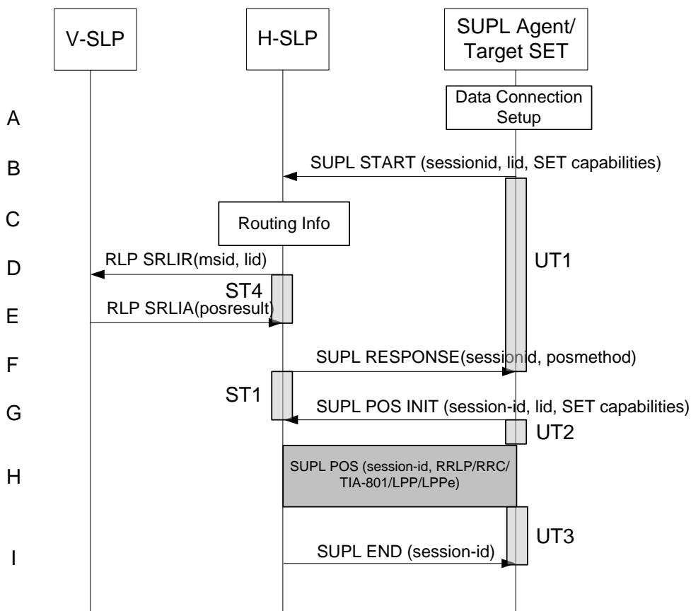
Figure 51: SET-Initiated Roaming with H-SLP Positioning Successful Case – Proxy mode
