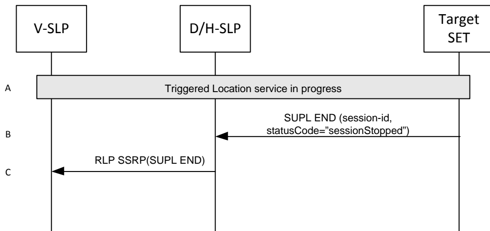
Figure 79: SET Initiated Event Trigger timer expiry
