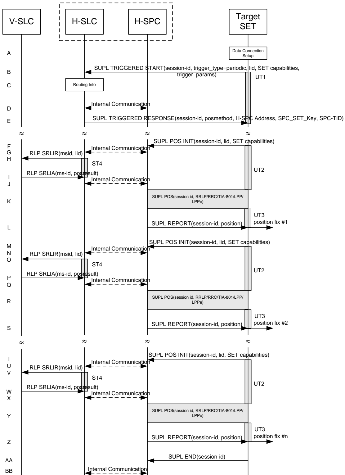
Figure 64: SET Initiated Periodic Trigger Service Roaming with H-SLP Positioning Successful Case – Non-Proxy Mode
