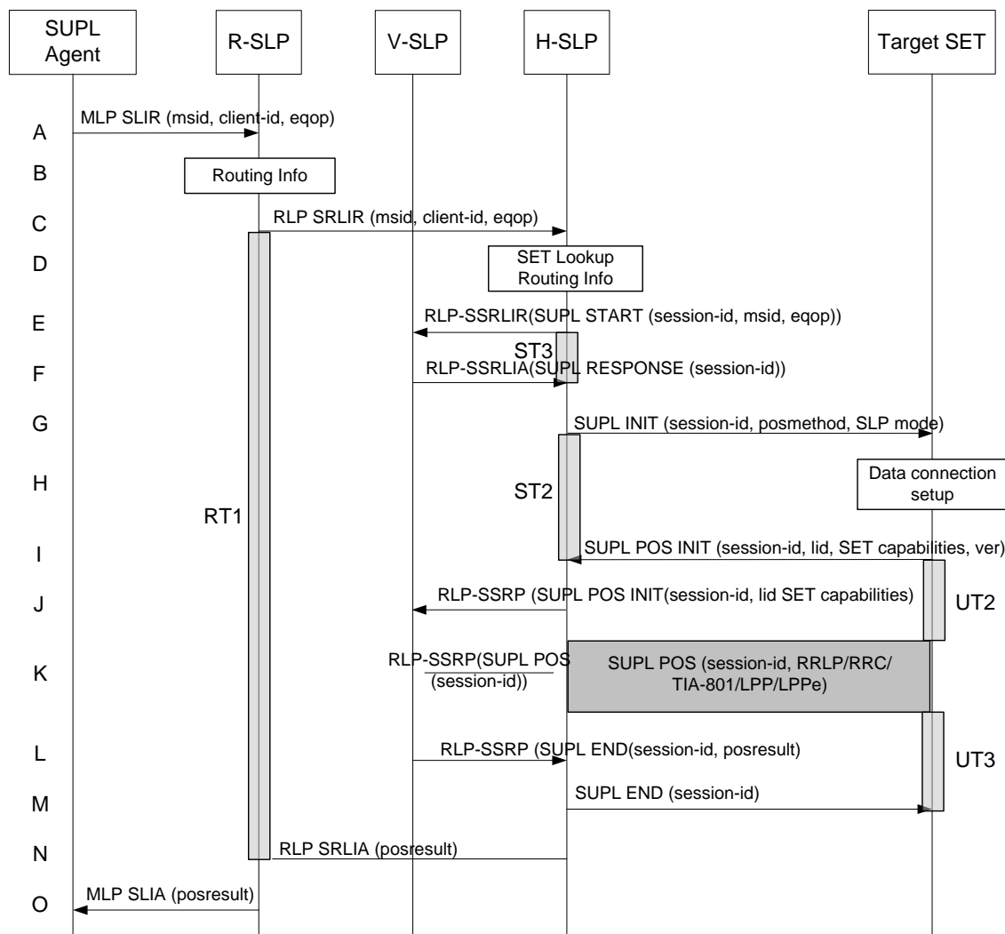
Figure 3: Network Initiated Roaming with V-SLP Positioning Successful Case – Proxy mode
