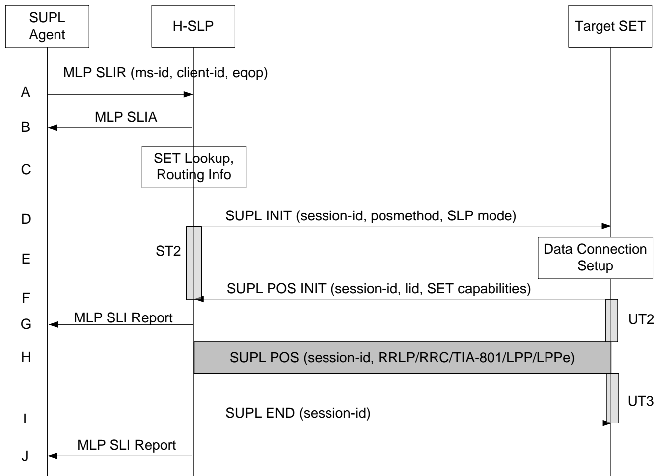
Figure 90: Network Initiated Non-Roaming Successful Case – Proxy Mode with asynchronous MLP request
