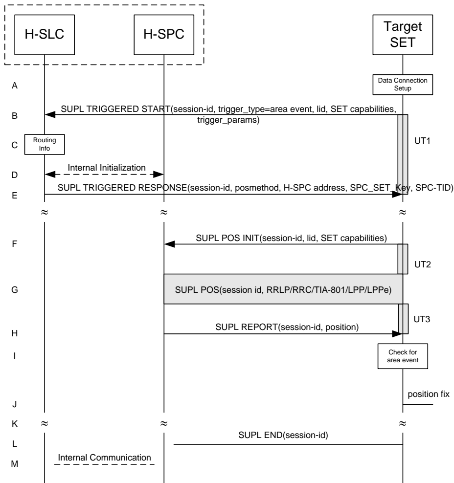
Figure 65: SET Initiated Area Event Trigger Service Non-Roaming Successful Case – Non-Proxy Mode
