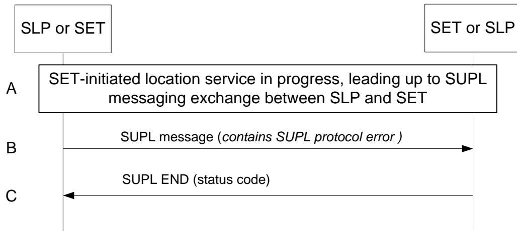
Figure 76: SET-Initiated Error SUPL Protocol Error
