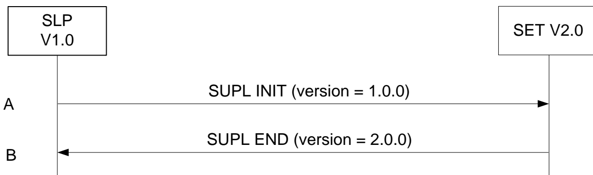
Figure 86: Network Initiated – SLP supports lower version than SET.
