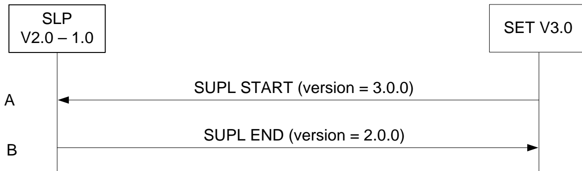
Figure 89: SET Initiated – SLP supports SUPL versions between 1.0 and 2.0 excluding requested version (V3.0).
