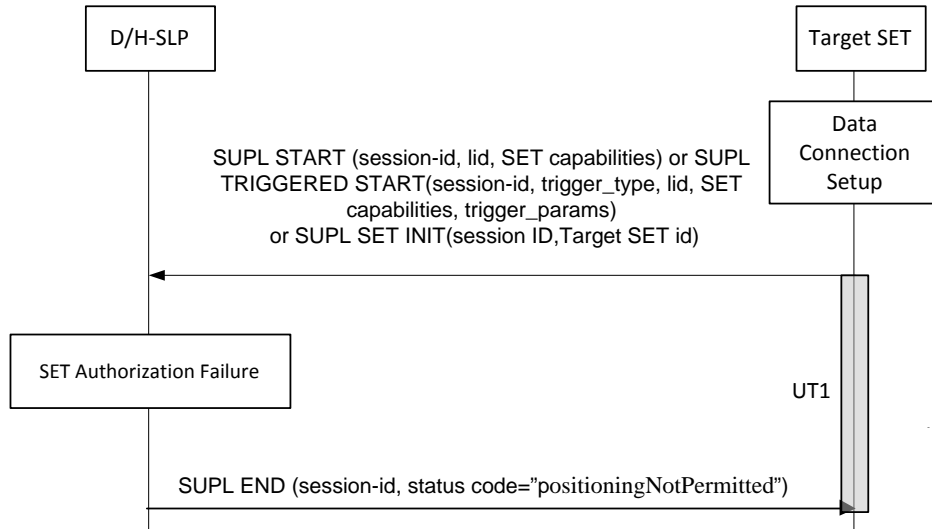
Figure 75: SET-Initiated Error SET Authorization Failure
