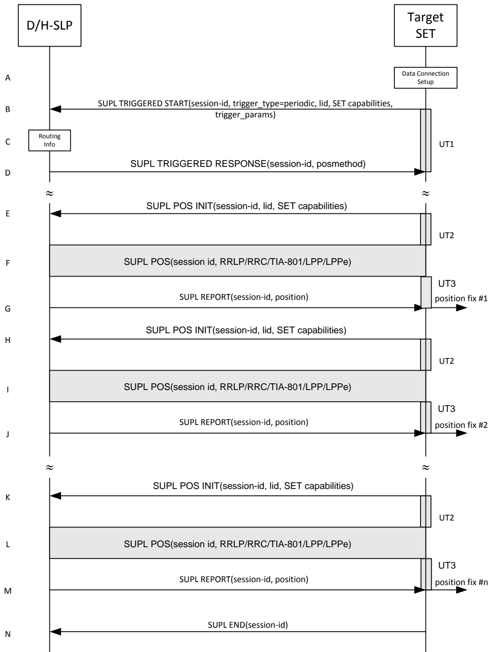
Figure 56: SET Initiated Periodic Trigger Service Non-Roaming Successful Case – Proxy Mode
