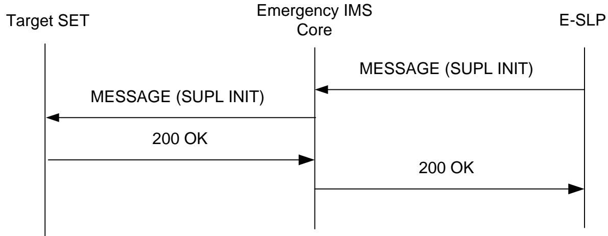
Figure 92: SIP Push Message Flow for IMS Emergency Location Services
