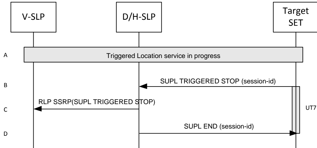
Figure 77: SET Initiated Triggered location, SET cancels the triggered location request
