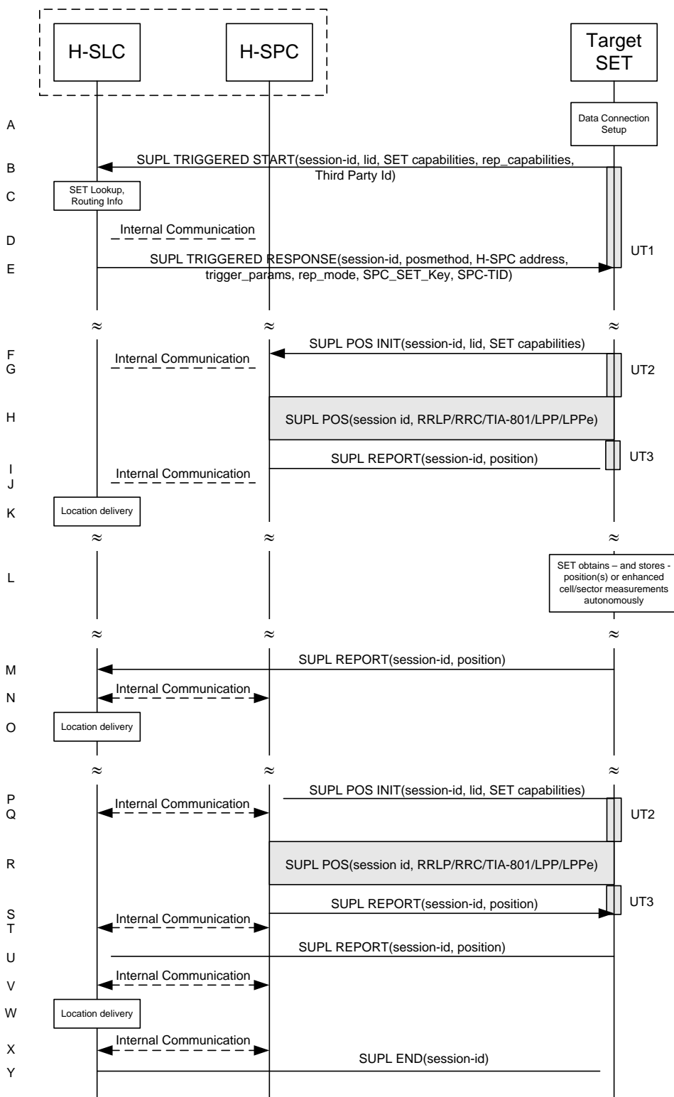
Figure 71: SET Initiated Periodic Location Request with transfer of the position result to 3rd party – non-roaming – non-proxy mode
