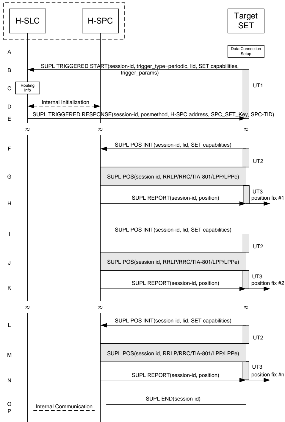
Figure 62: SET Initiated Periodic Trigger Service Non-Roaming Successful Case – Non-Proxy Mode
