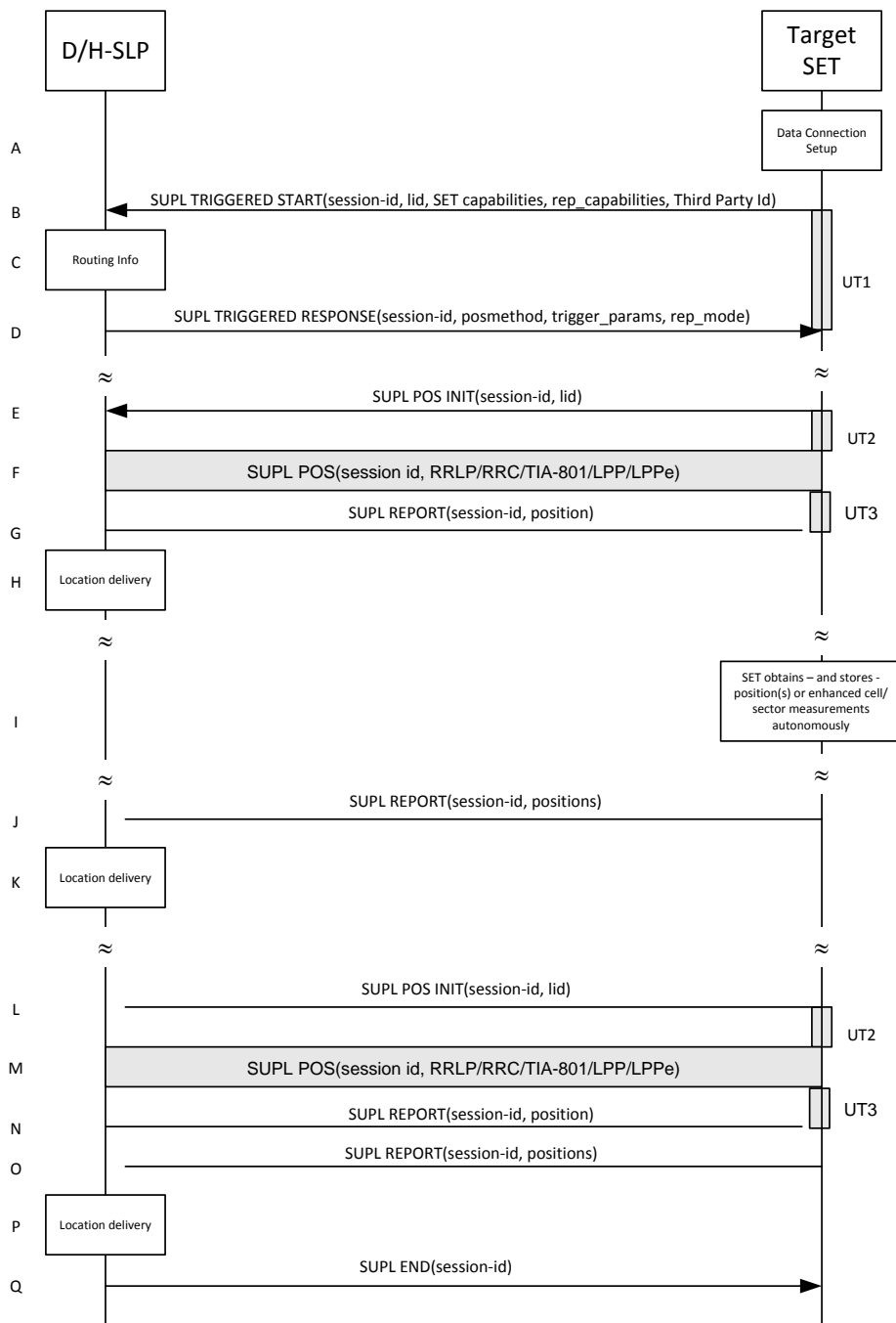
Figure 68: SET Initiated Periodic Location Request with transfer of the position result to 3rd party – non-roaming – proxy mode
