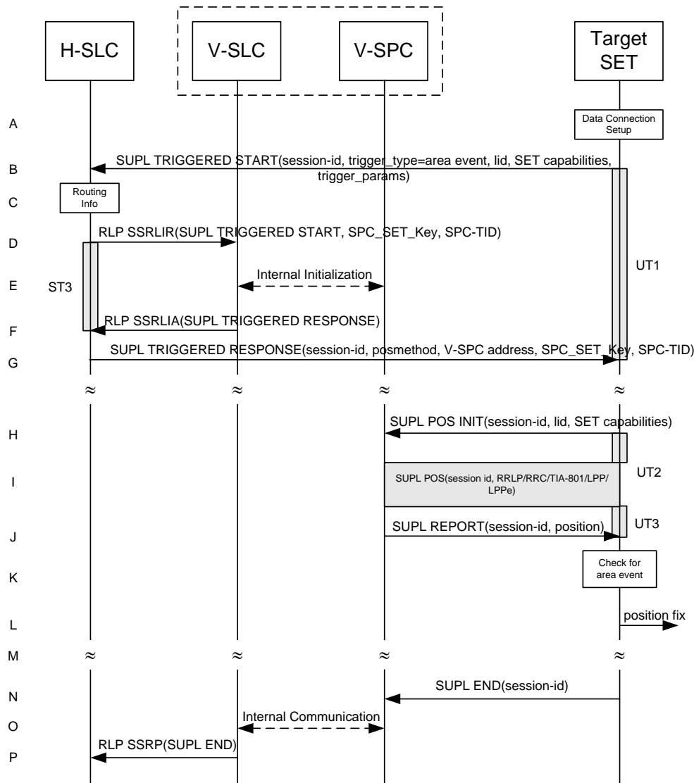
Figure 66: SET Initiated Area Event Trigger Service Roaming with V-SLP Positioning Successful Case – Non-Proxy Mode
