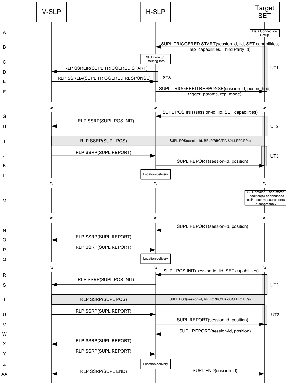
Figure 69: SET Initiated Periodic Location Request with transfer of the position result to 3rd party – roaming with V-SLP Positioning – proxy mode
