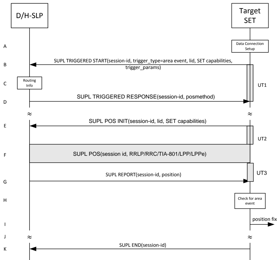
Figure 59: SET Initiated Area Event Trigger Service Non-Roaming Successful Case – Proxy Mode
