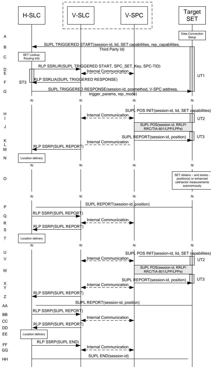
Figure 72: SET Initiated Periodic Location Request with transfer of the position result to 3rd party – roaming with V-SLP Positioning – non-proxy mode
