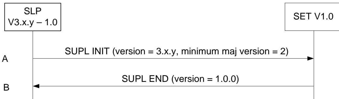
Figure 85: Network Initiated – SLP supports SUPL versions between 1.0 and 3.x.y but the requested service is not V1.0 compatible.
