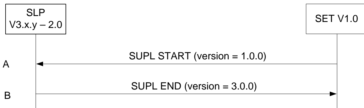
Figure 88: SET Initiated – SLP supports SUPL versions between 2.0 and 3.0 excluding requested version (V1.0).
