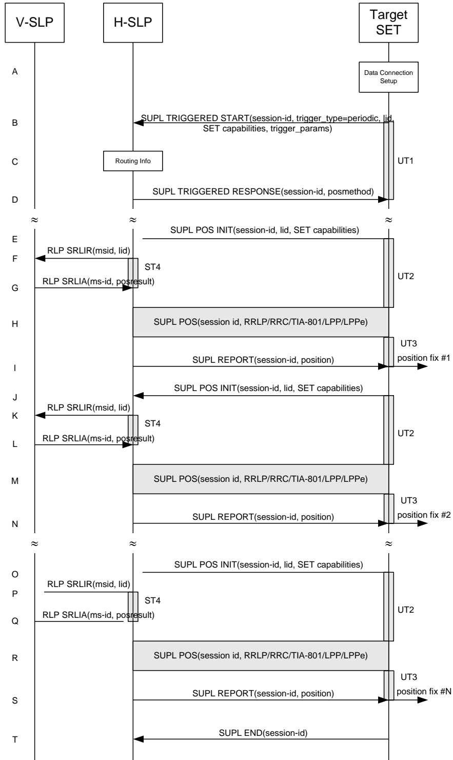
Figure 58: SET Initiated Periodic Trigger Service Roaming with H-SLP Positioning Successful Case – Proxy Mode
