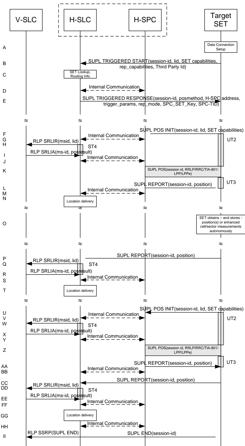
Figure 73: SET Initiated Periodic Location Request with transfer of the position result to 3rd party – roaming with H-SLP Positioning – non-proxy mode
