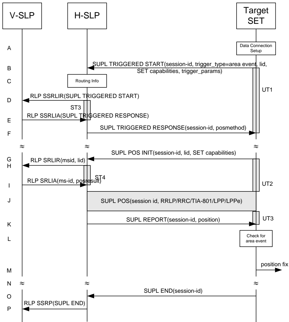
Figure 61: SET Initiated Area Event Trigger Service Roaming with H-SLP Positioning Successful Case – Proxy Mode
