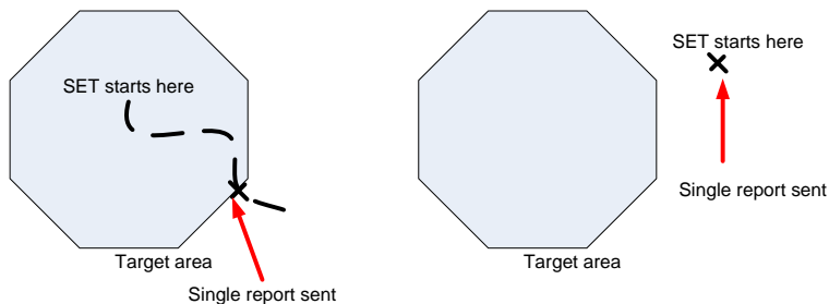
Figure 94: Single report when SET is outside area
