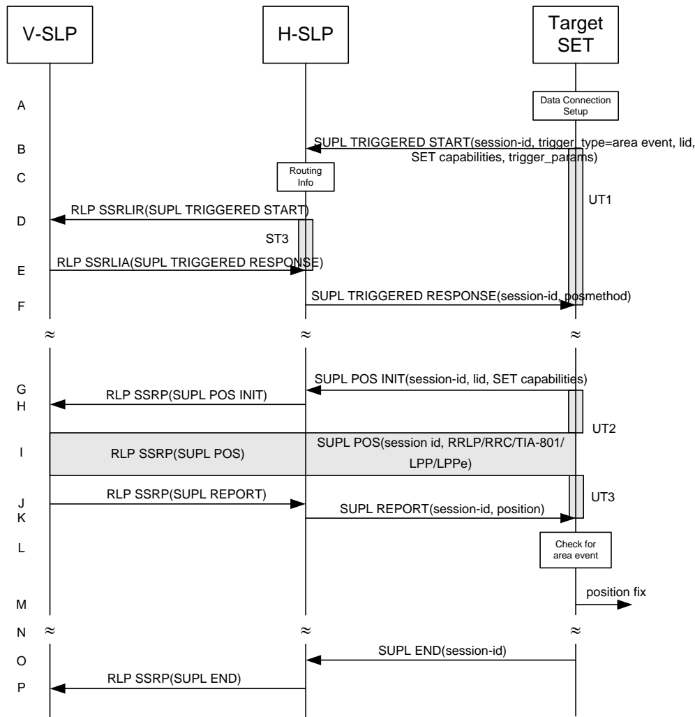
Figure 60: SET Initiated Area Event Trigger Service Roaming with V-SLP Positioning Successful Case – Proxy Mode
