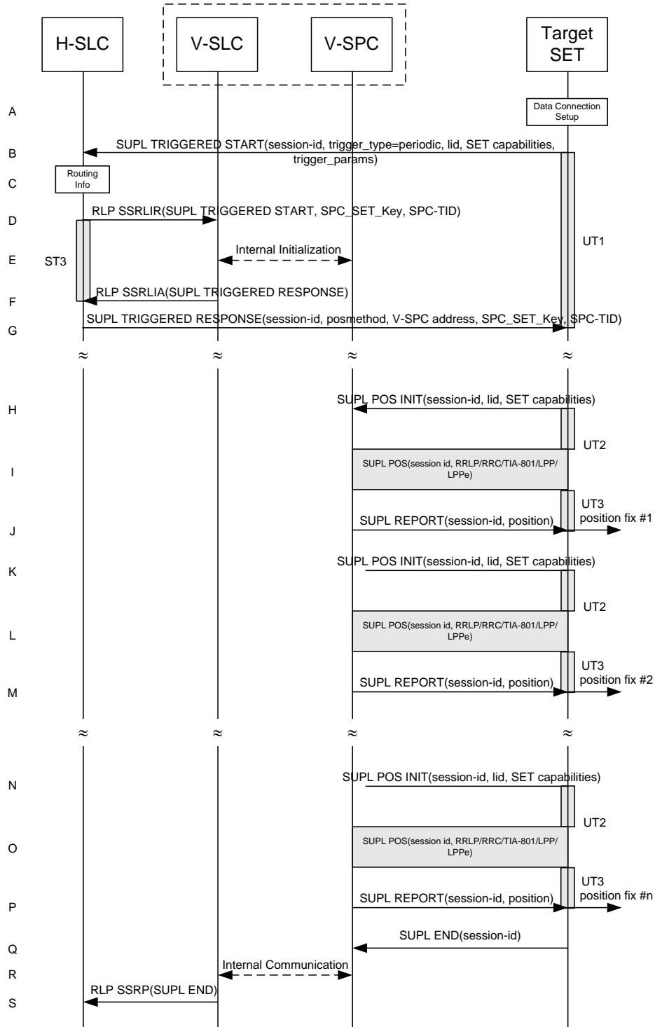
Figure 63: SET Initiated Periodic Trigger Service Roaming with V-SLP Positioning Successful Case – Non-Proxy Mode
