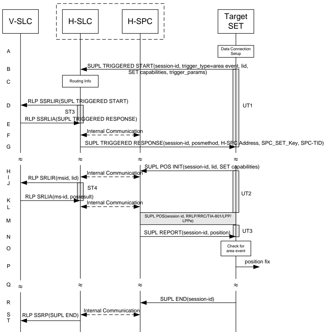
Figure 67: SET Initiated Area Event Trigger Service Roaming with H-SLP Positioning Successful Case – Non-Proxy Mode
