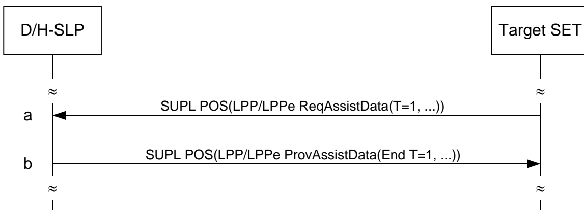
Figure 61: LPP/LPPE Assistance Data Transfer Procedure
