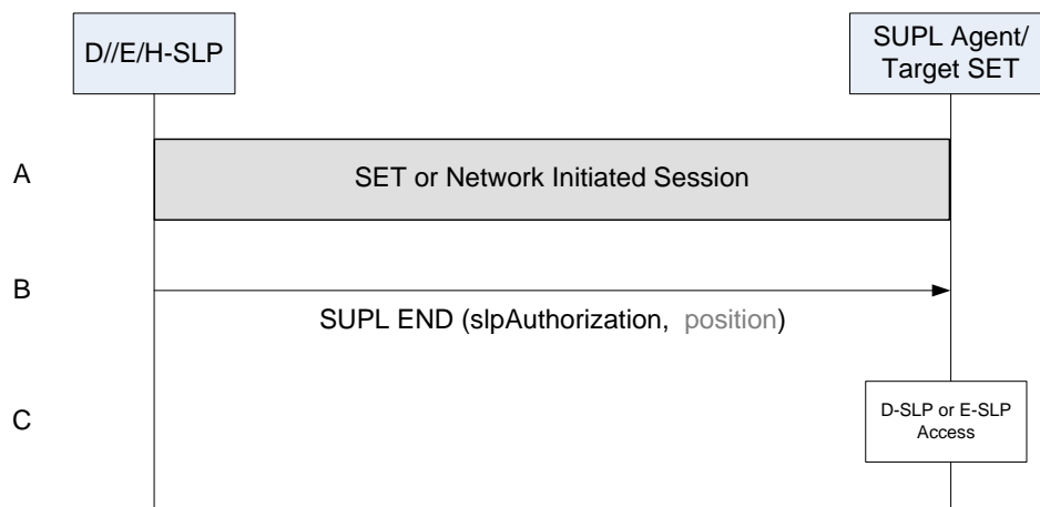
Figure 12: Unsolicited Authorization of D-SLPs and E-SLPs by a an H-SLP, Proxy D-SLP or Proxy E-SLP
