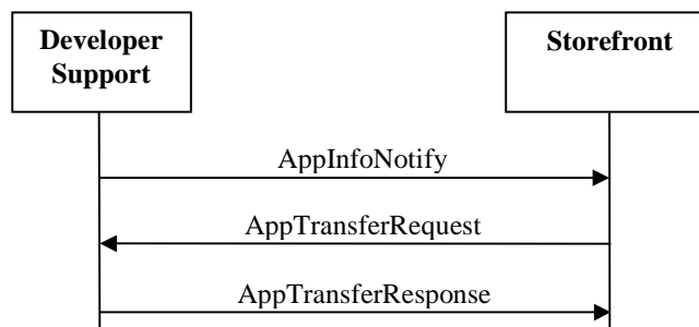
Figure 4: Application Transfer messages exchange
