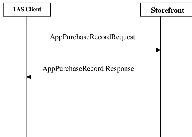
Figure 26: Application Purchase Record Messages Exchange
