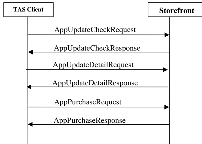
Figure 18: Application Update messages exchange
