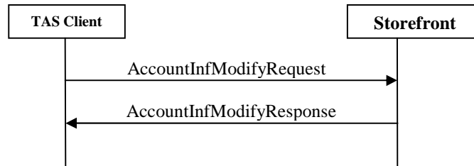
Figure 16: User Account information modification messages exchange
