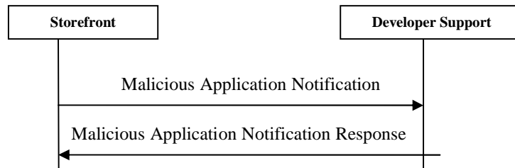
Figure 45: Malicious Application Notification Messages Exchange
