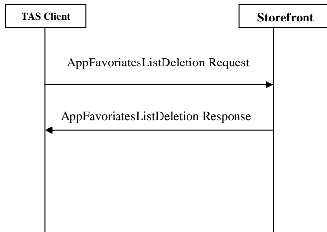
Figure 28: Application Faroriates List Deletion Messages Exchange
