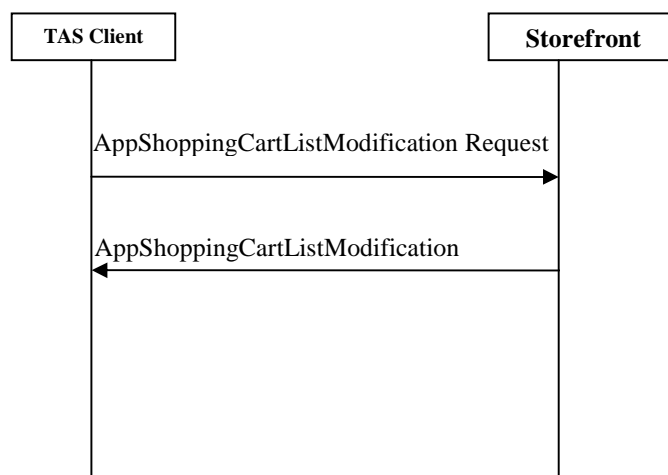
Figure 34: AppShoppingCartListModification Messages Exchange
