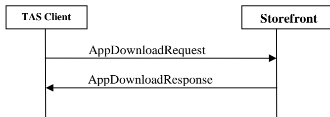
Figure 10: Application Download messages exchange
