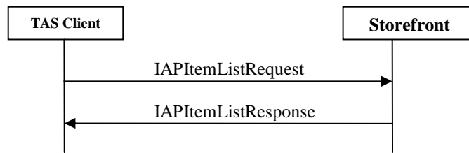
Figure 35: IAP Item List messages exchange
