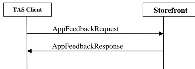
Figure 12: Application Feedback messages exchange
