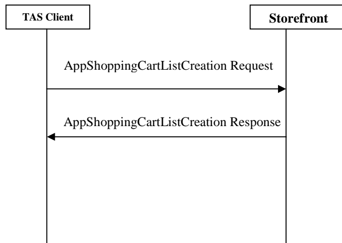
Figure 33: AppShoppingCartListCreation Messages Exchange
