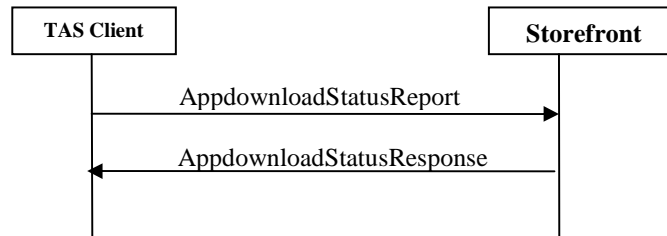
Figure 23: Application Download Status Report messages exchange
