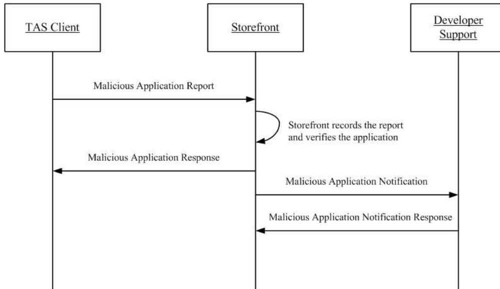
Figure 51: Malicious Application Report Flow
