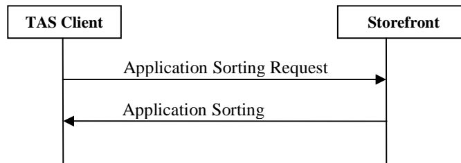
Figure 19: Application Sorting messages exchange
