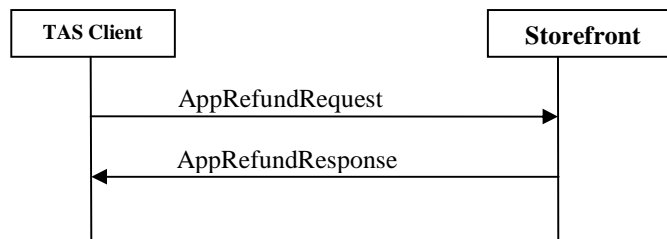
Figure 22: Application Refund messages exchange
