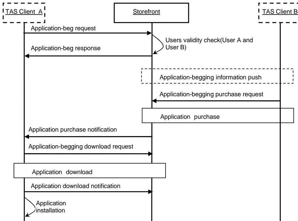
Figure 53: Application Begging Flow
