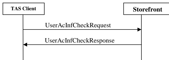
Figure 15: User Account Information Check messages exchange
