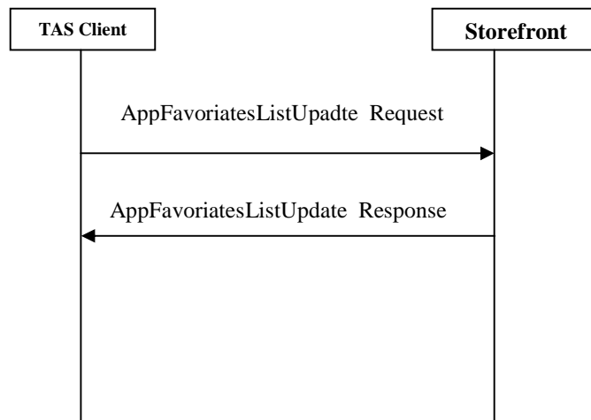
Figure 29: Application Favorites List Update Messages Exchange
