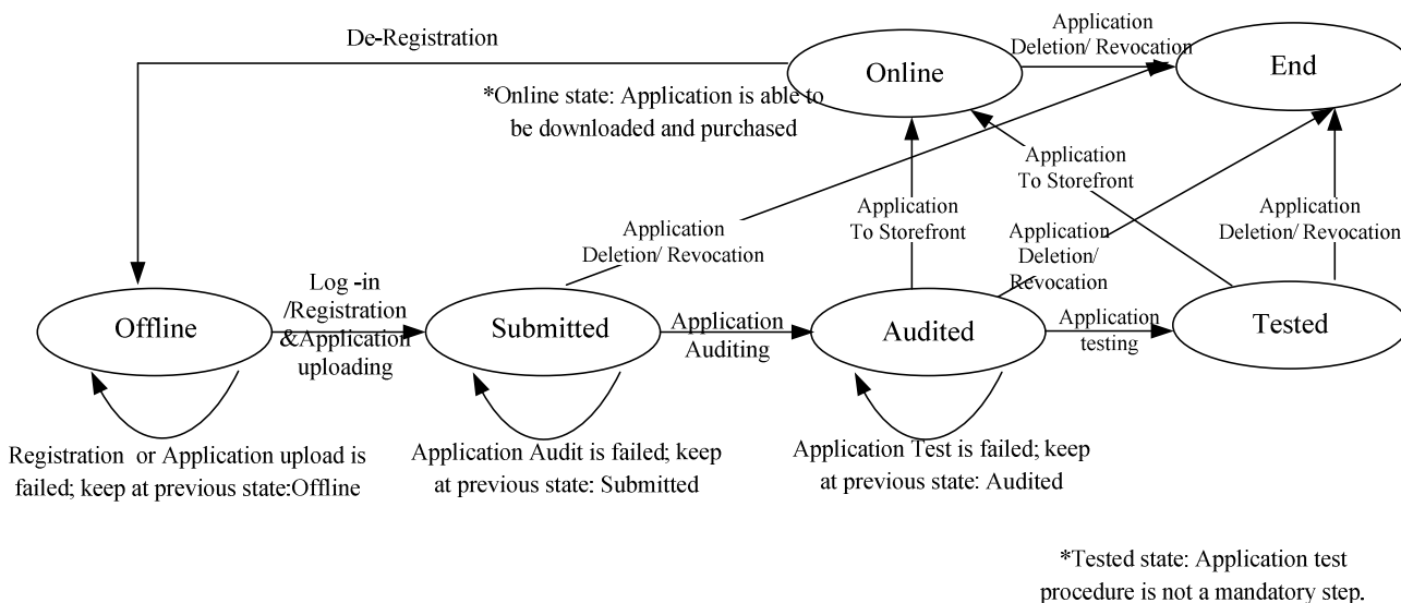
Figure 2: Application State Flow Control
