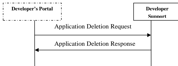
Figure 39: Application Deletion messages exchange
