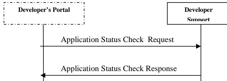
Figure 40: Application Status Check Messages exchange
