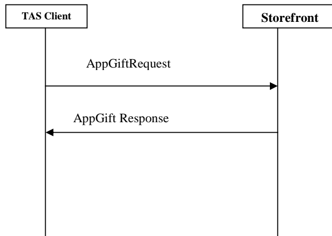
Figure 30: Application Gift Messages Exchange
