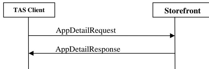
Figure 24: Application Detail messages exchange
