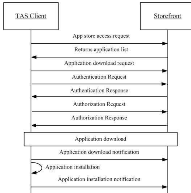
Figure 49: Application Download Flow
