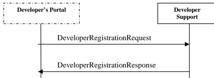
Figure 43: Application Sales Report messages exchange
