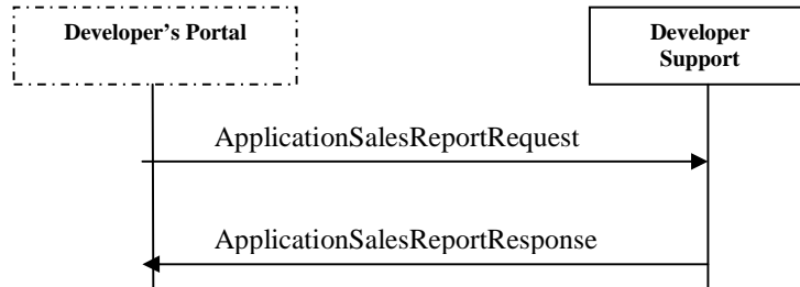
Figure 42: Application Sales Report messages exchange
