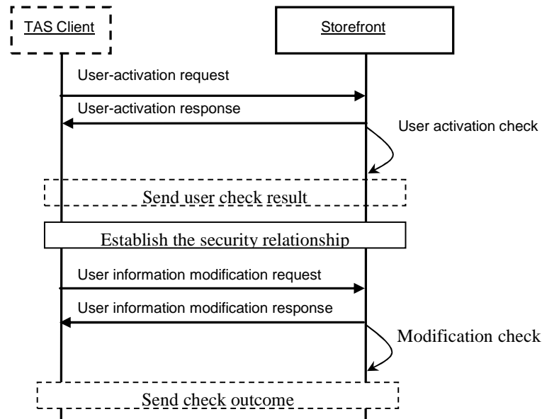
Figure 54: User Activation and Modification Flow
