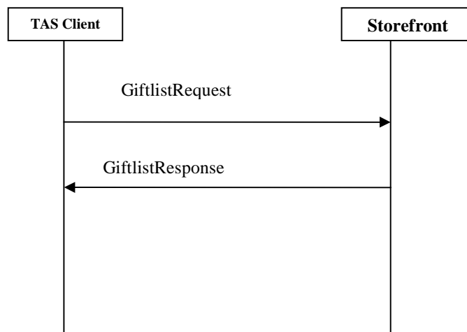
Figure 32: Gift Reception Messages Exchange
