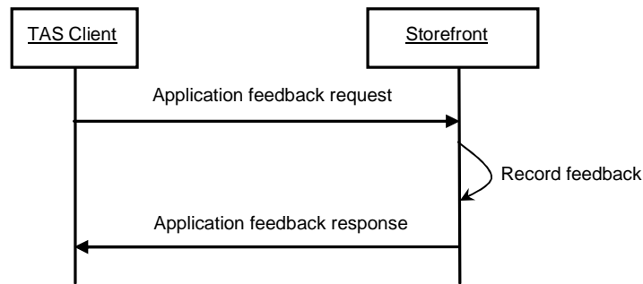
Figure 50: Application Feedback Flow
