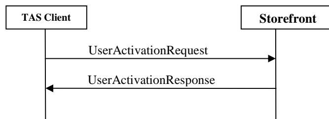
Figure 13: User Activation messages exchange
