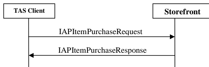
Figure 36: IAP Item Purchase messages exchange
