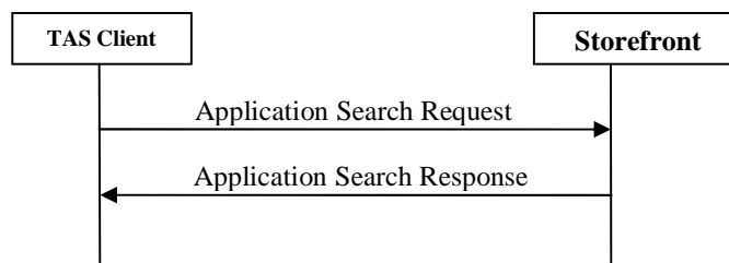
Figure 20: Application Search messages exchange
