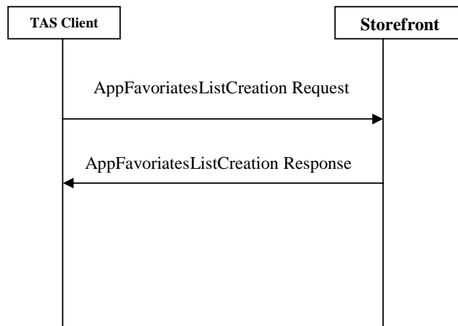
Figure 27: Application Favourites List Creation Messages Exchange
