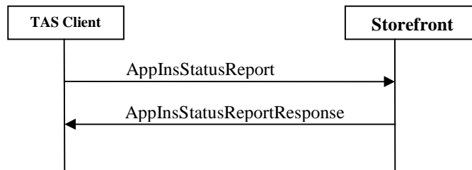
Figure 14: Application Install Status Report messages exchange
