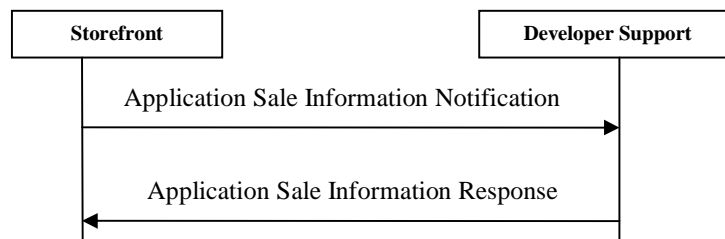
Figure 46: Application Sale Information message exchange
