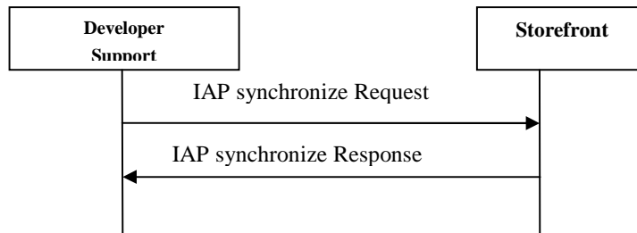
Figure 8: IAP synchronize messages exchange
