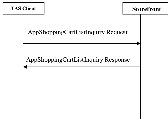
Figure 37: AppShoppingCartListInquiry Messages Exchange
