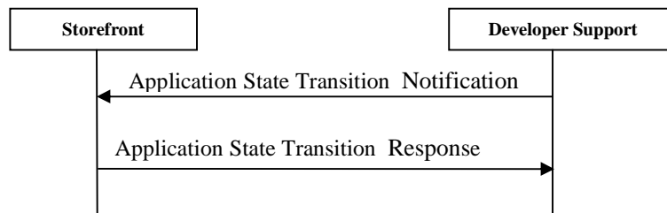
Figure 7: Application state transition Notification messages exchange
