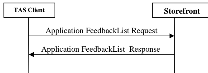
Figure 25: Application FeedbackList messages exchange
