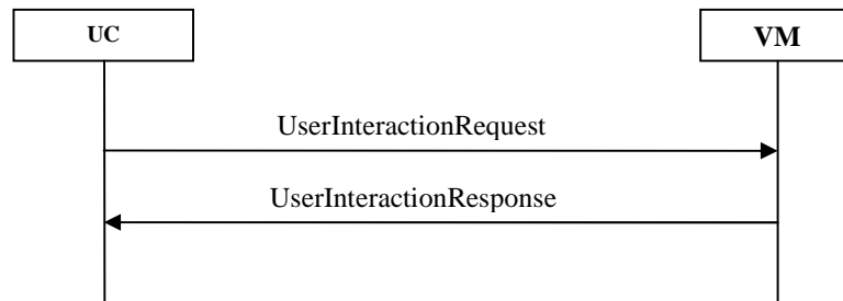
Figure 15: Flow of UserInteractionRequest and its response
