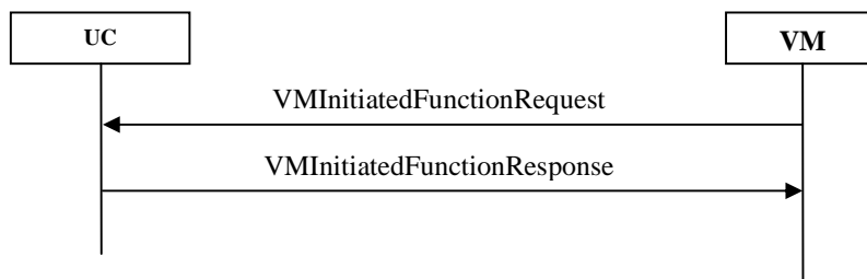
Figure 19: Flow of VMInitiatedFunctionRequest and its response
