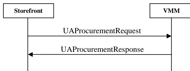
Figure 26: Flow of UAProcurementRequest and its response
