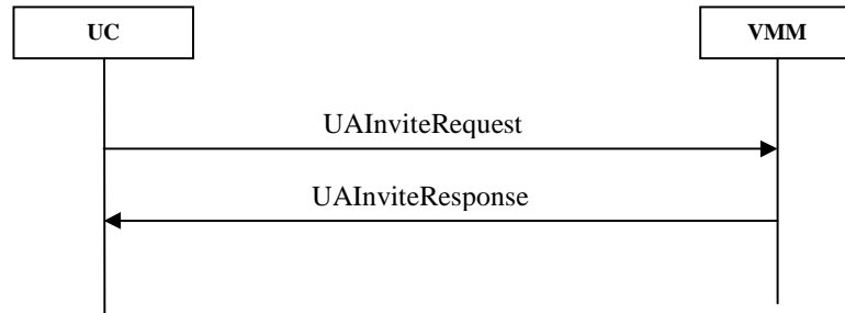
Figure 8: Flow of UAINVITE Message Exchange
