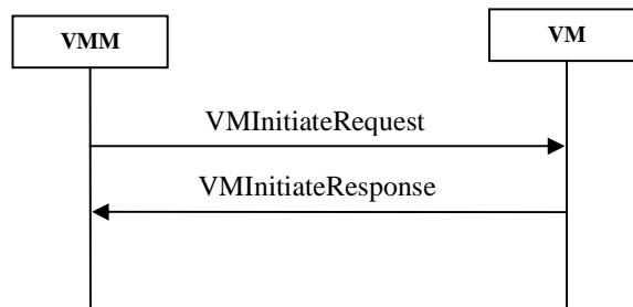
Figure 11: Flow of VMInitiateRequest and its response
