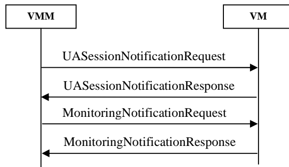
Figure 13: Flow of two Notification request and their response
