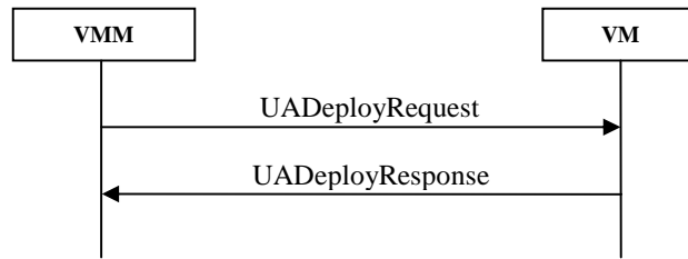
Figure 12: Flow of UADeployRequest and its response
