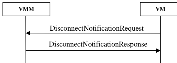
Figure 21: Flow of DisconnectNotificationRequest and its response
