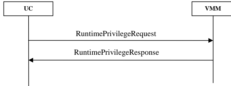
Figure 9: Flow of runtime privilege request
