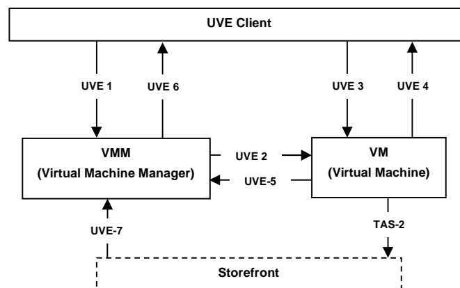
Figure 2: Architectural Diagram
