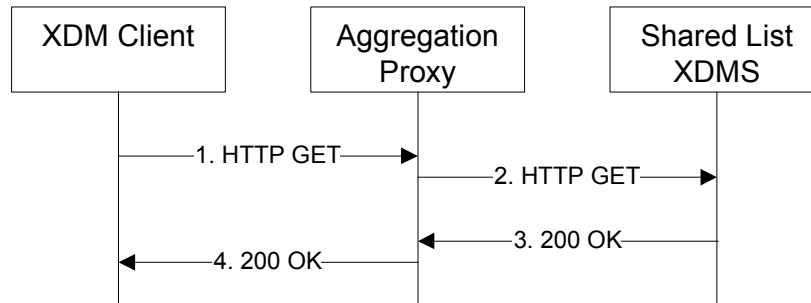
Figure C.1.2 XDMC obtains Group Usage Lists
