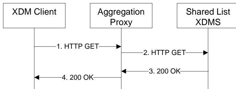
Figure C.1.2 XDMC obtains Group Usage Lists
