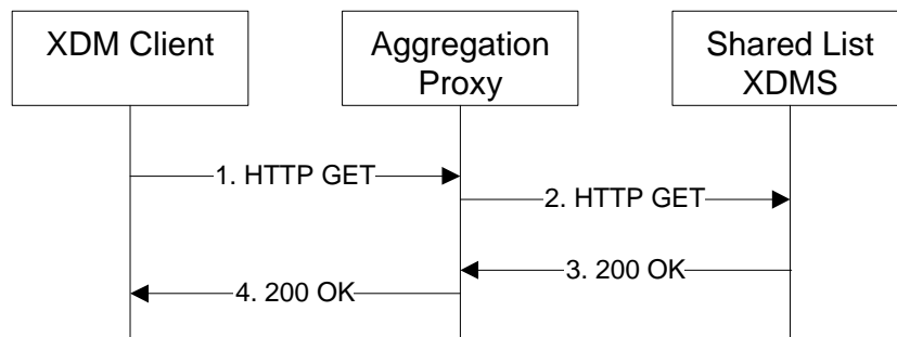
Figure C.1.1 XDMC obtains URI Lists
