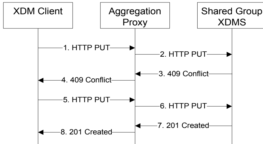
Figure C.2- Group XDMS negotiates a Conference URI
