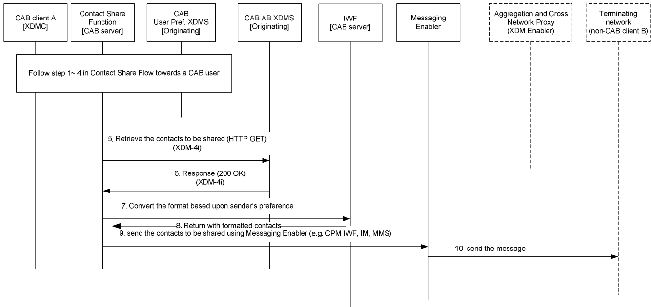
Figure 9 : Flows of Contact Share towards a non CAB user
