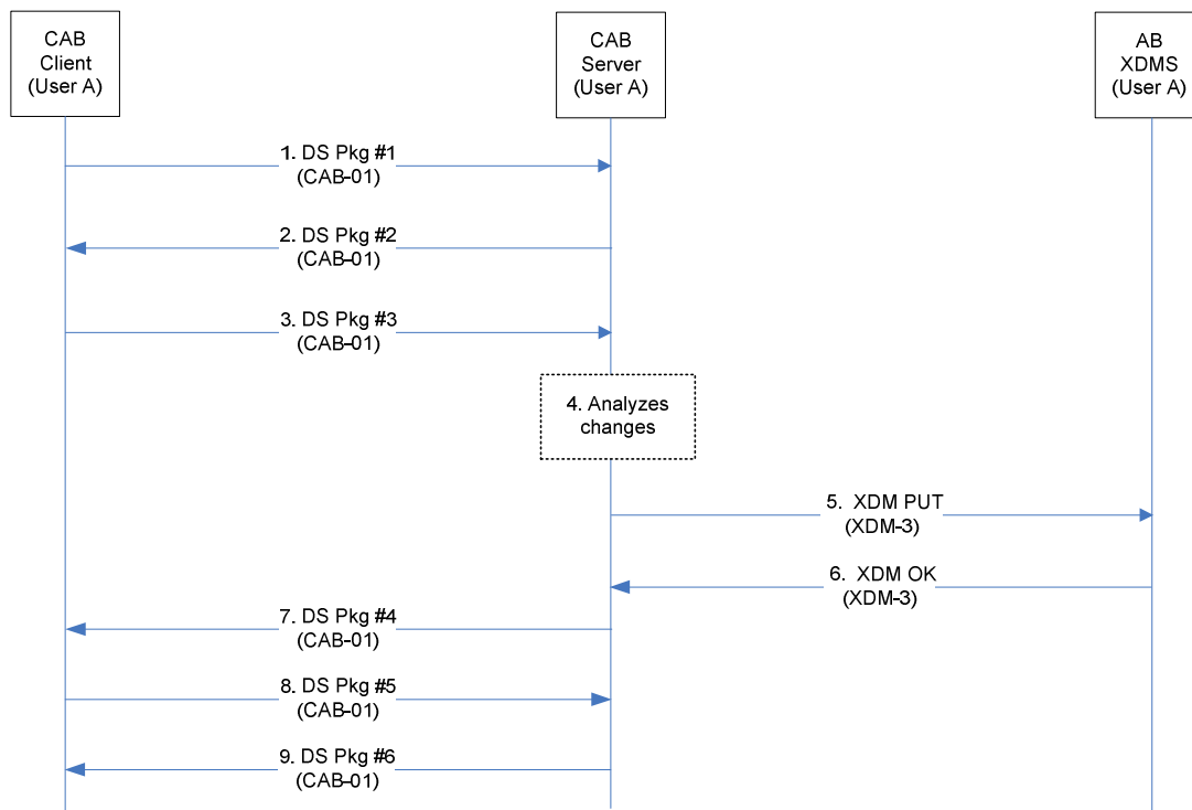
Figure 11 : CAB Client Address Book Modifications and Synchronization Flow
