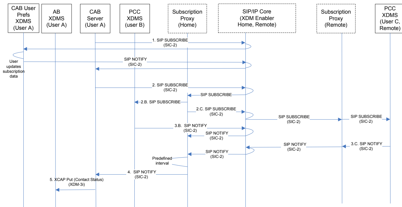
Figure 10 : Contact Subscription flow using the Subscription Proxy
