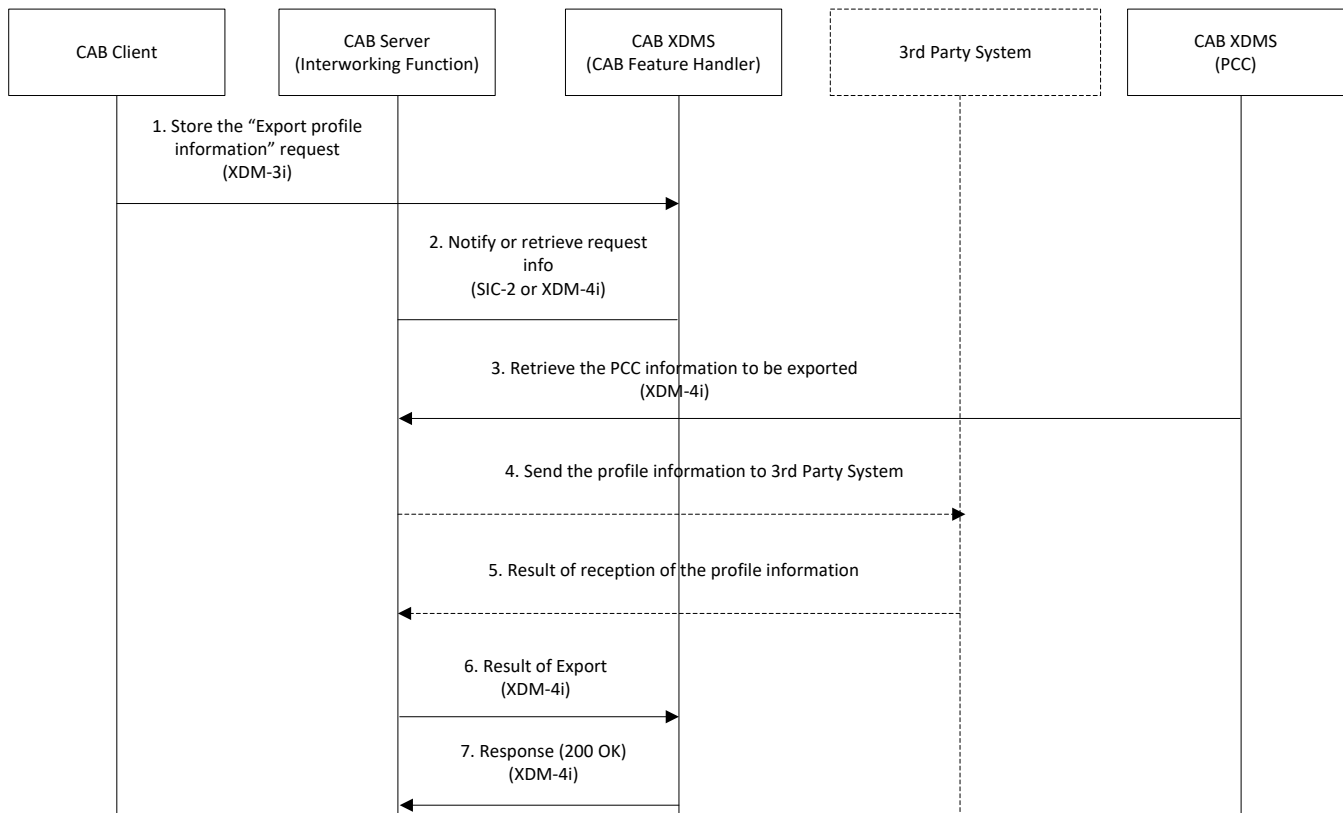
Figure 22 : PCC Information Export Flows
