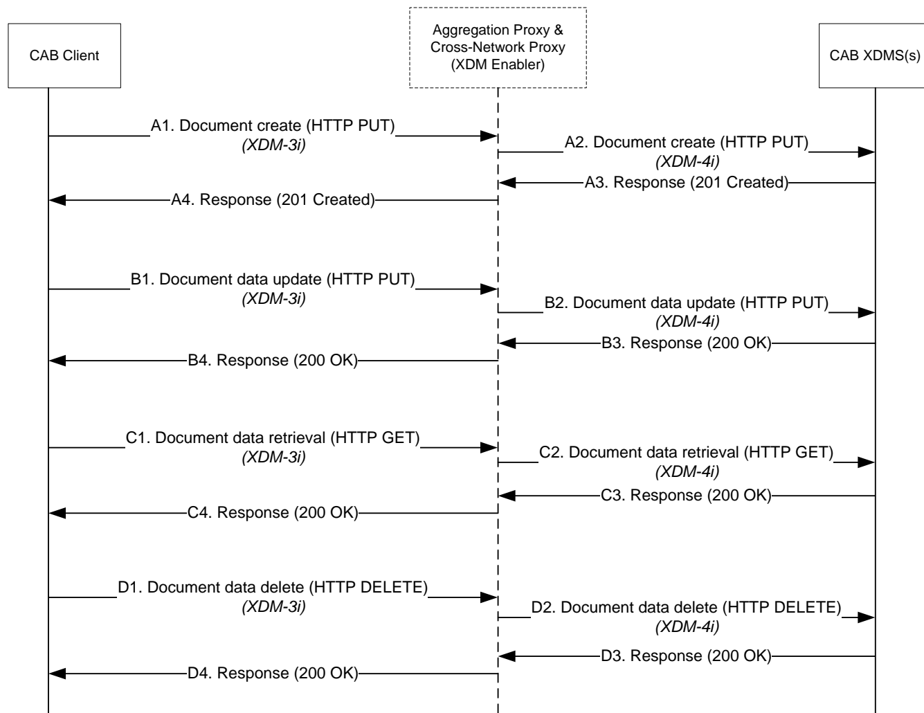
Figure 6: CAB Client manipulating a CAB XML document
