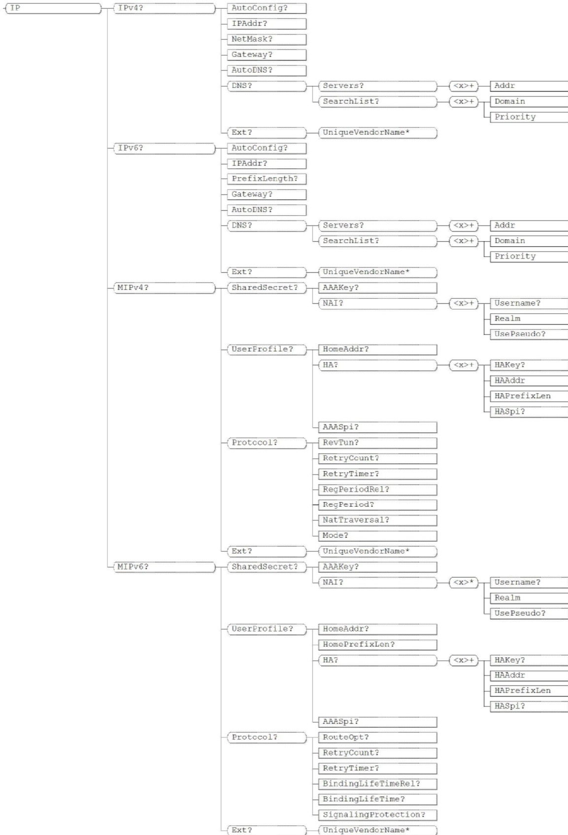
Figure 2: Continuation of NAP Management Object (Informative)
