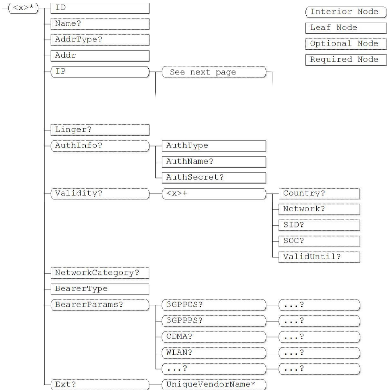
Figure 1: NAP Management Object (Informative)
